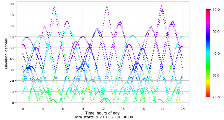
Time-elevation plot for station VIGO. Signal to Noise S1C Data file VIGO00ESP_R_2023332.xtr
