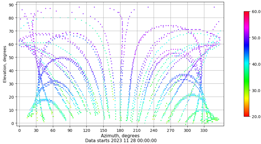
Azimuth-elevation plot for station VIGO. Signal to Noise S1C Data file VIGO00ESP_R_2023332.xtr
