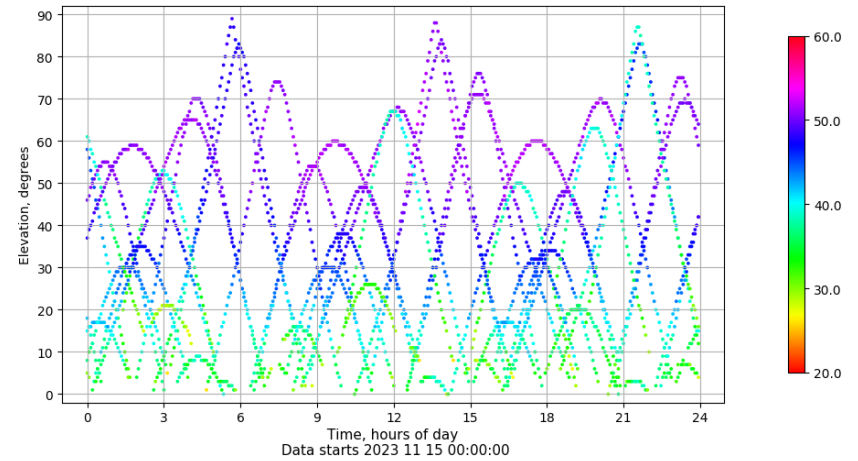
Time-elevation plot for station VIGO. Signal to Noise S1C Data file VIGO00ESP_R_2023319.xtr
