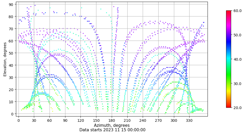
Azimuth-elevation plot for station VIGO. Signal to Noise S1C Data file VIGO00ESP_R_2023319.xtr
