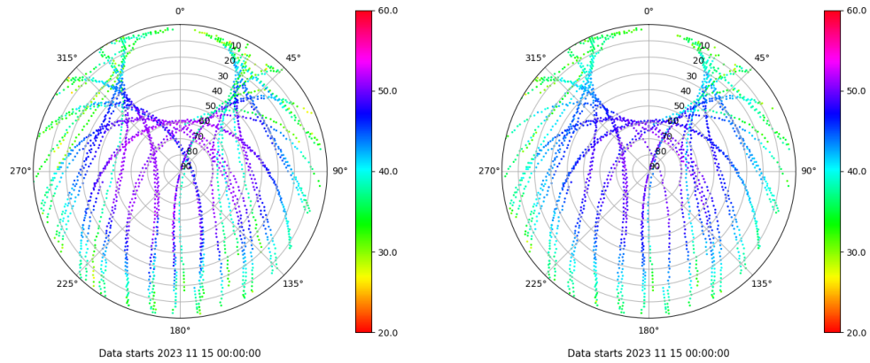
Skyplot for station VIGO. Signal to Noise S1C Data file VIGO00ESP_R_2023319.xtr Skyplot for station VIGO. Signal to Noise S2C Data file VIGO00ESP_R_2023319.xtr
