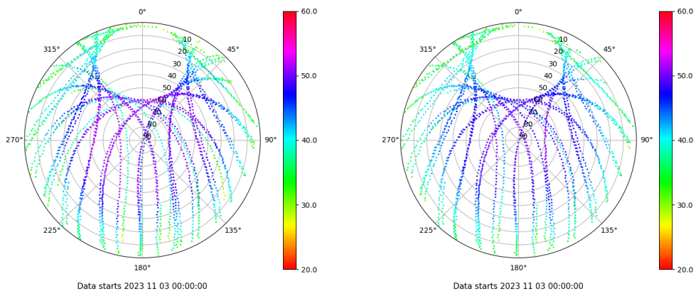
Skyplot for station VIGO. Signal to Noise S1C Data file VIGO00ESP_R_2023307.xtr Skyplot for station VIGO. Signal to Noise S2C Data file VIGO00ESP_R_2023307.xtr
