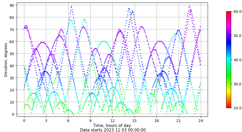
Time-elevation plot for station VIGO. Signal to Noise S1C Data file VIGO00ESP_R_2023307.xtr
