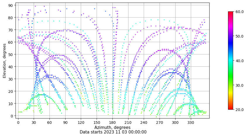
Azimuth-elevation plot for station VIGO. Signal to Noise S1C Data file VIGO00ESP_R_2023307.xtr
