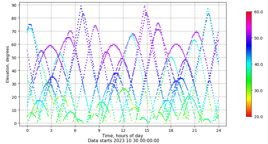
Time-elevation plot for station VIGO. Signal to Noise S1C Data file VIGO00ESP_R_2023303.xtr
