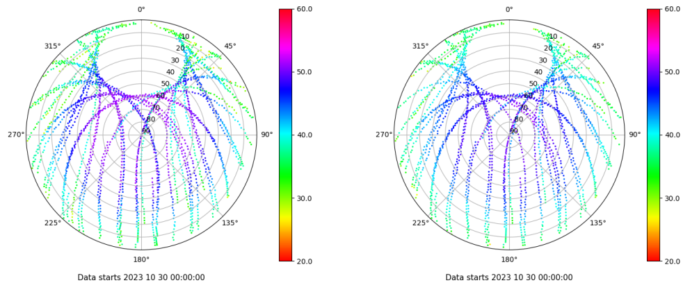
Skyplot for station VIGO. Signal to Noise S1C Data file VIGO00ESP_R_2023303.xtr Skyplot for station VIGO. Signal to Noise S2C Data file VIGO00ESP_R_2023303.xtr
