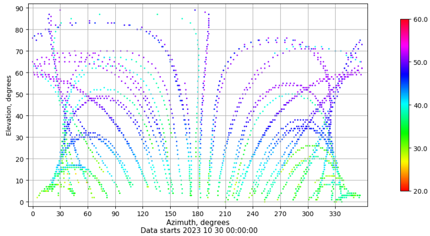
Azimuth-elevation plot for station VIGO. Signal to Noise S1C Data file VIGO00ESP_R_2023303.xtr
