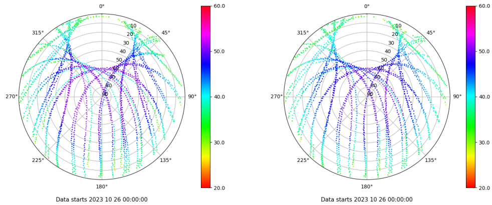
Skyplot for station VIGO. Signal to Noise S1C Data file VIGO00ESP_R_2023299.xtr Skyplot for station VIGO. Signal to Noise S2C Data file VIGO00ESP_R_2023299.xtr
