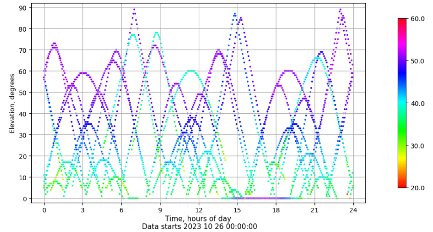
Time-elevation plot for station VIGO. Signal to Noise S1C Data file VIGO00ESP_R_2023299.xtr
