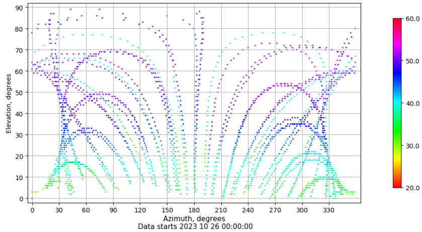
Azimuth-elevation plot for station VIGO. Signal to Noise S1C Data file VIGO00ESP_R_2023299.xtr
