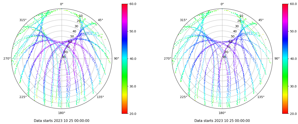
Skyplot for station VIGO. Signal to Noise S1C Data file VIGO00ESP_R_2023298.xtr Skyplot for station VIGO. Signal to Noise S2C Data file VIGO00ESP_R_2023298.xtr
