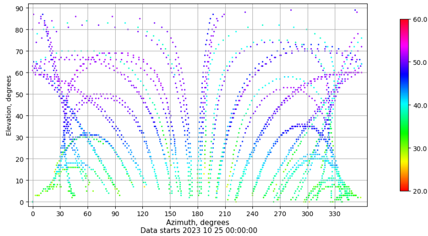
Azimuth-elevation plot for station VIGO. Signal to Noise S1C Data file VIGO00ESP_R_2023298.xtr
