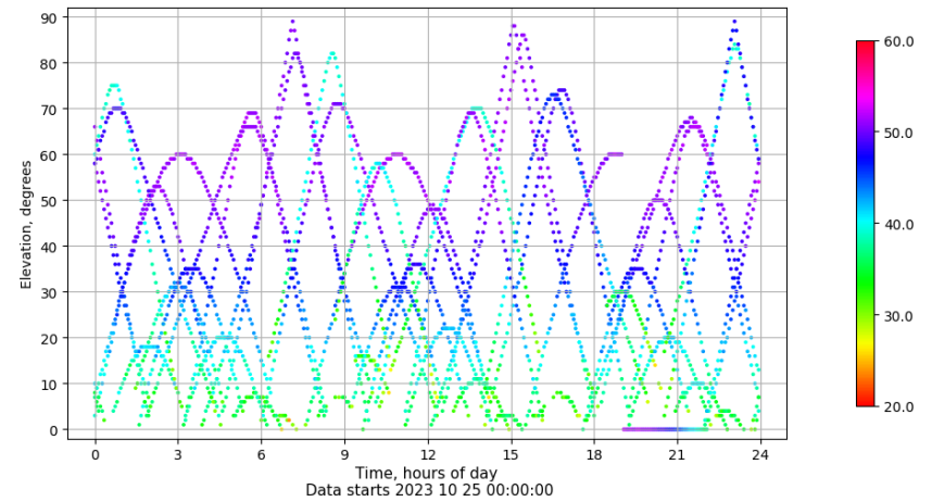
Time-elevation plot for station VIGO. Signal to Noise S1C Data file VIGO00ESP_R_2023298.xtr
