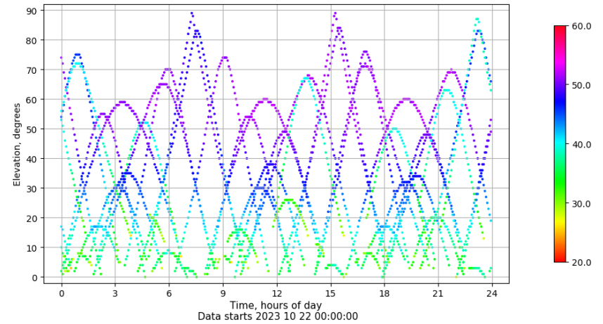
Time-elevation plot for station VIGO. Signal to Noise S1C Data file VIGO00ESP_R_2023295.xtr
