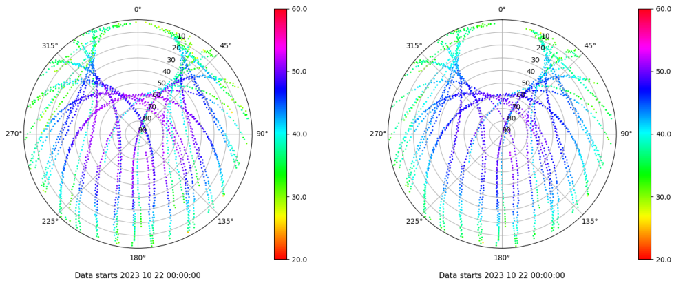
Skyplot for station VIGO. Signal to Noise S1C Data file VIGO00ESP_R_2023295.xtr Skyplot for station VIGO. Signal to Noise S2C Data file VIGO00ESP_R_2023295.xtr
