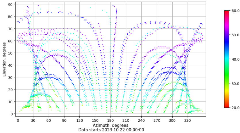
Azimuth-elevation plot for station VIGO. Signal to Noise S1C Data file VIGO00ESP_R_2023295.xtr
