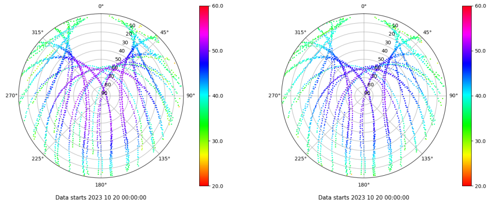
Skyplot for station VIGO. Signal to Noise S1C Data file VIGO00ESP_R_2023293.xtr Skyplot for station VIGO. Signal to Noise S2C Data file VIGO00ESP_R_2023293.xtr
