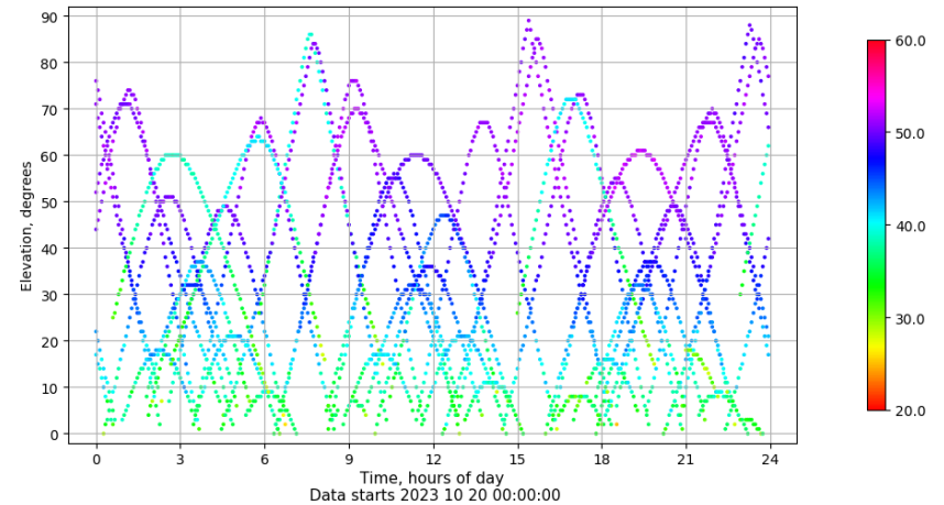
Time-elevation plot for station VIGO. Signal to Noise S1C Data file VIGO00ESP_R_2023293.xtr
