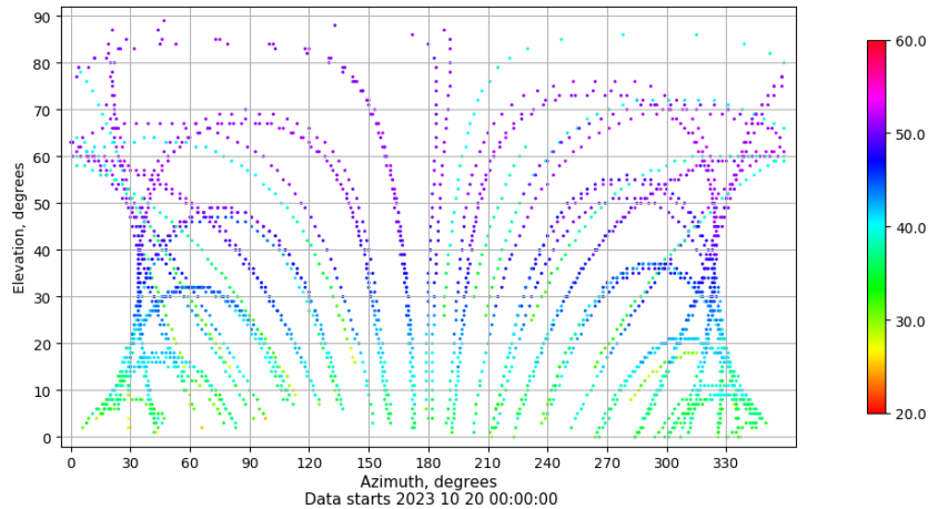
Azimuth-elevation plot for station VIGO. Signal to Noise S1C Data file VIGO00ESP_R_2023293.xtr
