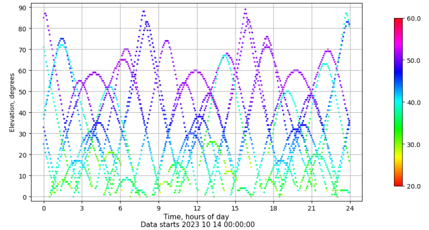
Time-elevation plot for station VIGO. Signal to Noise S1C Data file VIGO00ESP_R_2023287.xtr
