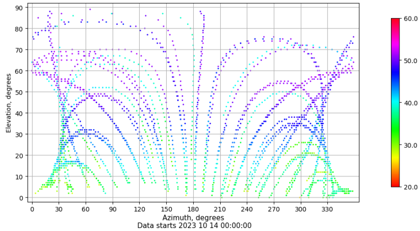
Azimuth-elevation plot for station VIGO. Signal to Noise S1C Data file VIGO00ESP_R_2023287.xtr
