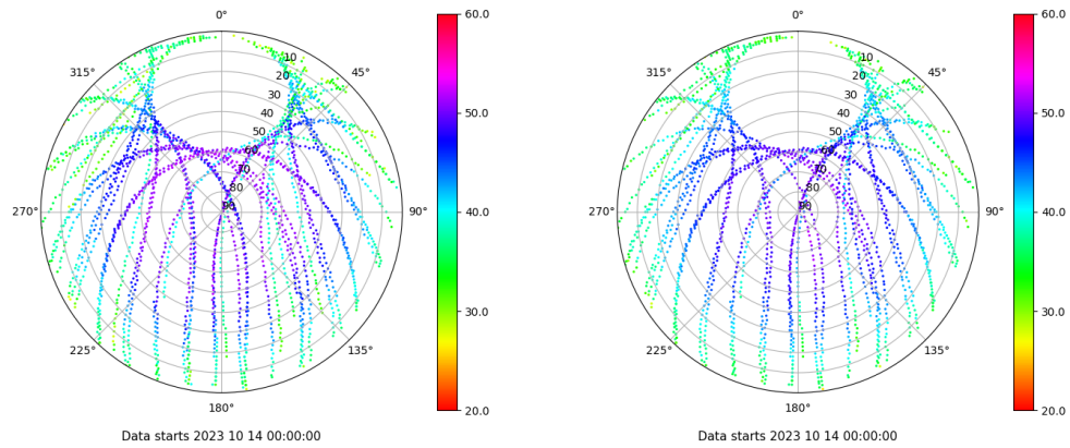
Skyplot for station VIGO. Signal to Noise S1C Data file VIGO00ESP_R_2023287.xtr Skyplot for station VIGO. Signal to Noise S2C Data file VIGO00ESP_R_2023287.xtr
