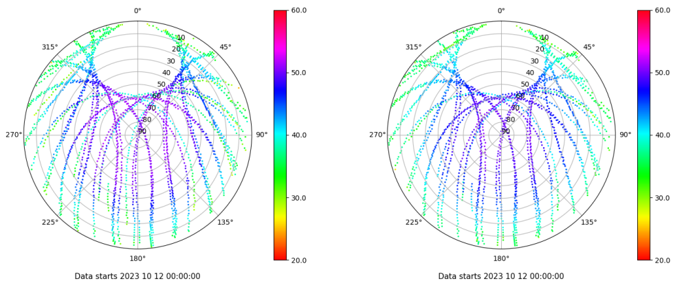
Skyplot for station VIGO. Signal to Noise S1C Data file VIGO00ESP_R_2023285.xtr Skyplot for station VIGO. Signal to Noise S2C Data file VIGO00ESP_R_2023285.xtr
