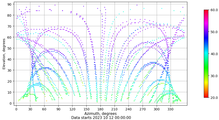
Azimuth-elevation plot for station VIGO. Signal to Noise S1C Data file VIGO00ESP_R_2023285.xtr
