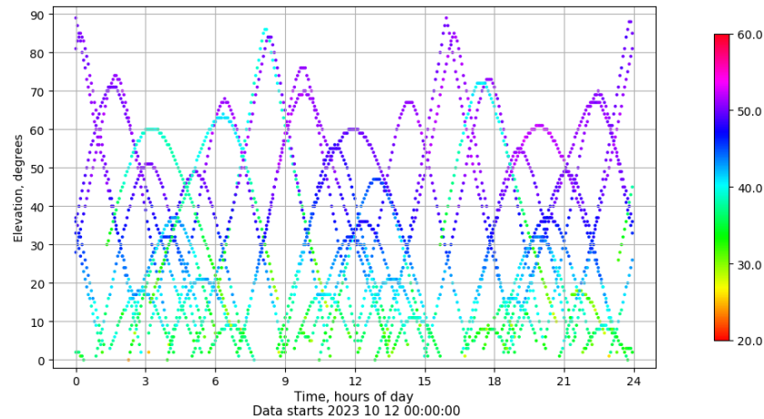
Time-elevation plot for station VIGO. Signal to Noise S1C Data file VIGO00ESP_R_2023285.xtr
