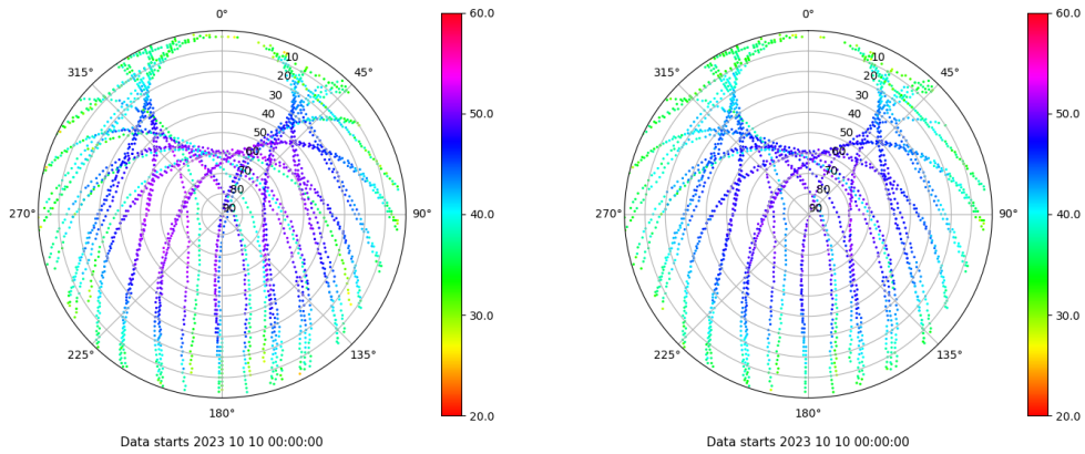
Skyplot for station VIGO. Signal to Noise S1C Data file VIGO00ESP_R_2023283.xtr Skyplot for station VIGO. Signal to Noise S2C Data file VIGO00ESP_R_2023283.xtr
