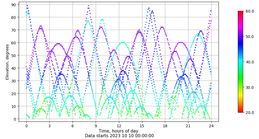
Time-elevation plot for station VIGO. Signal to Noise S1C Data file VIGO00ESP_R_2023283.xtr
