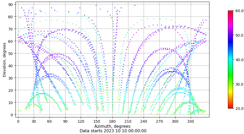
Azimuth-elevation plot for station VIGO. Signal to Noise S1C Data file VIGO00ESP_R_2023283.xtr
