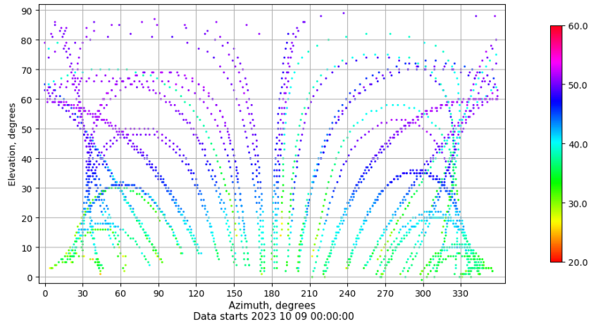
Azimuth-elevation plot for station VIGO. Signal to Noise S1C Data file VIGO00ESP_R_2023282.xtr
