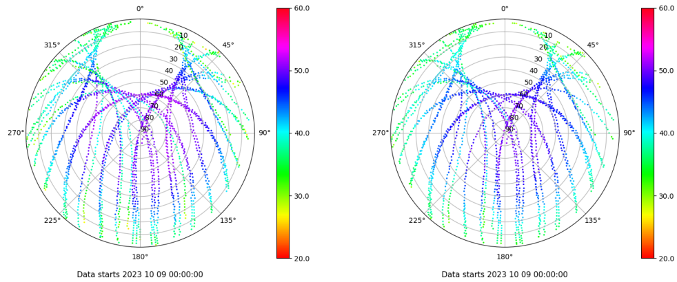
Skyplot for station VIGO. Signal to Noise S1C Data file VIGO00ESP_R_2023282.xtr Skyplot for station VIGO. Signal to Noise S2C Data file VIGO00ESP_R_2023282.xtr
