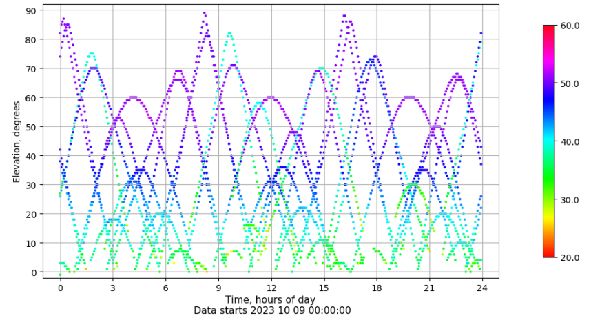
Time-elevation plot for station VIGO. Signal to Noise S1C Data file VIGO00ESP_R_2023282.xtr
