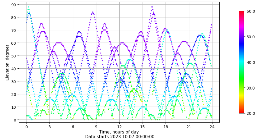
Time-elevation plot for station VIGO. Signal to Noise S1C Data file VIGO00ESP_R_2023280.xtr
