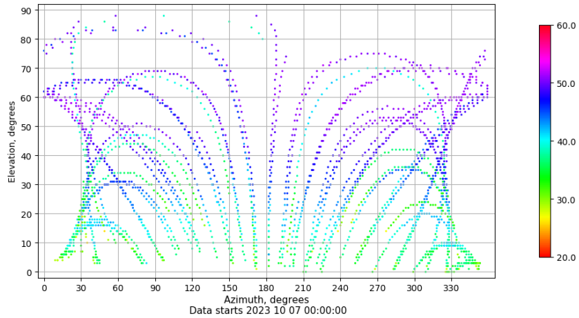
Azimuth-elevation plot for station VIGO. Signal to Noise S1C Data file VIGO00ESP_R_2023280.xtr
