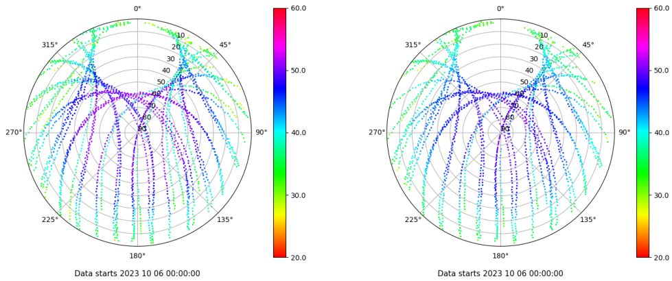
Skyplot for station VIGO. Signal to Noise S1C Data file VIGO00ESP_R_2023279.xtr Skyplot for station VIGO. Signal to Noise S2C Data file VIGO00ESP_R_2023279.xtr
