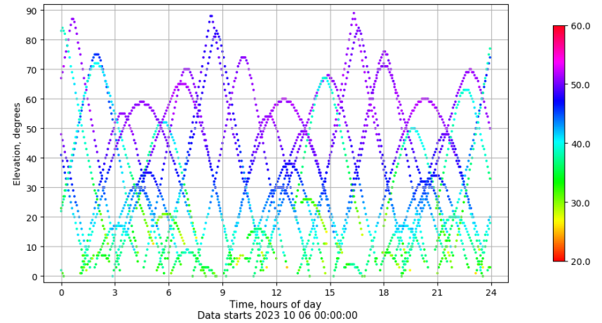
Time-elevation plot for station VIGO. Signal to Noise S1C Data file VIGO00ESP_R_2023279.xtr
