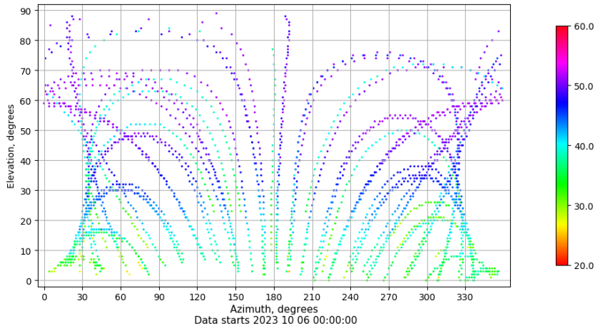
Azimuth-elevation plot for station VIGO. Signal to Noise S1C Data file VIGO00ESP_R_2023279.xtr
