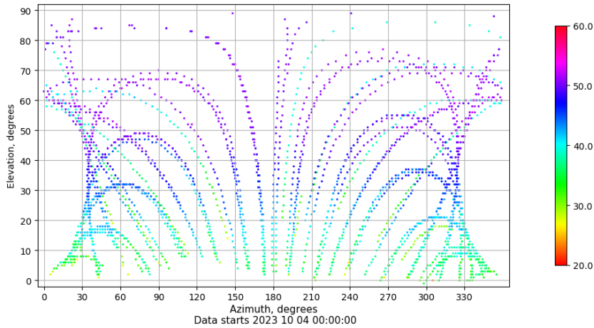
Azimuth-elevation plot for station VIGO. Signal to Noise S1C Data file VIGO00ESP_R_2023277.xtr
