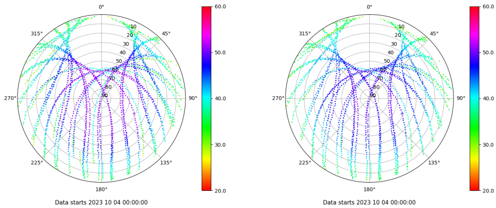
Skyplot for station VIGO. Signal to Noise S1C Data file VIGO00ESP_R_2023277.xtr Skyplot for station VIGO. Signal to Noise S2C Data file VIGO00ESP_R_2023277.xtr
