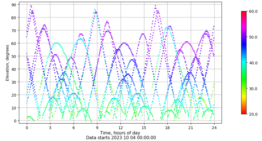
Time-elevation plot for station VIGO. Signal to Noise S1C Data file VIGO00ESP_R_2023277.xtr
