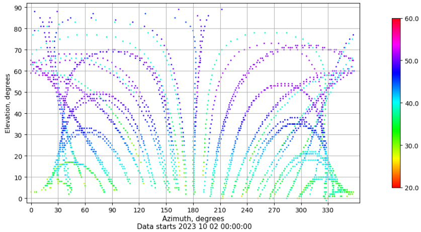
Azimuth-elevation plot for station VIGO. Signal to Noise S1C Data file VIGO00ESP_R_2023275.xtr
