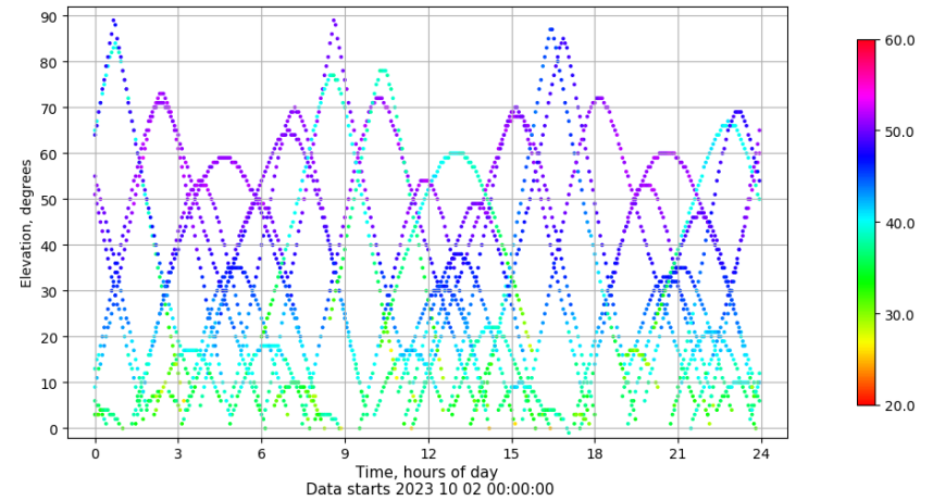
Time-elevation plot for station VIGO. Signal to Noise S1C Data file VIGO00ESP_R_2023275.xtr
