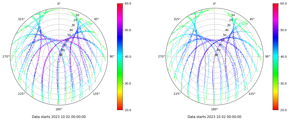
Skyplot for station VIGO. Signal to Noise S1C Data file VIGO00ESP_R_2023275.xtr Skyplot for station VIGO. Signal to Noise S2C Data file VIGO00ESP_R_2023275.xtr
