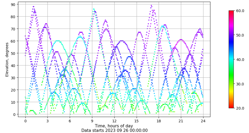
Time-elevation plot for station VIGO. Signal to Noise S1C Data file VIGO00ESP_R_2023269.xtr
