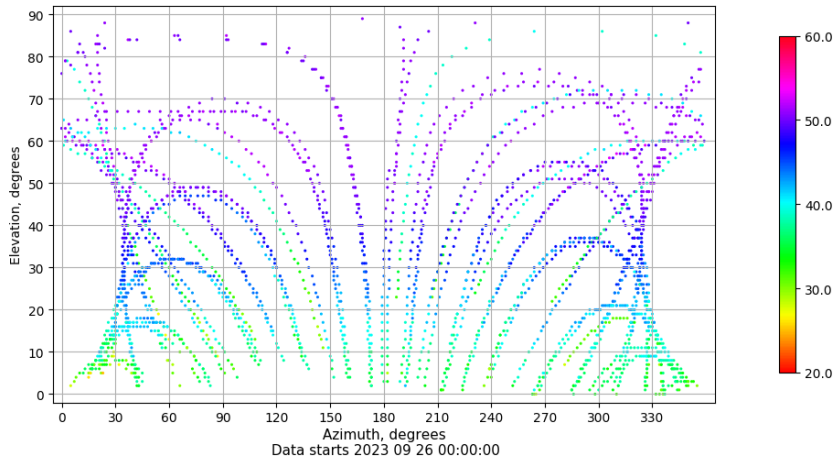
Azimuth-elevation plot for station VIGO. Signal to Noise S1C Data file VIGO00ESP_R_2023269.xtr
