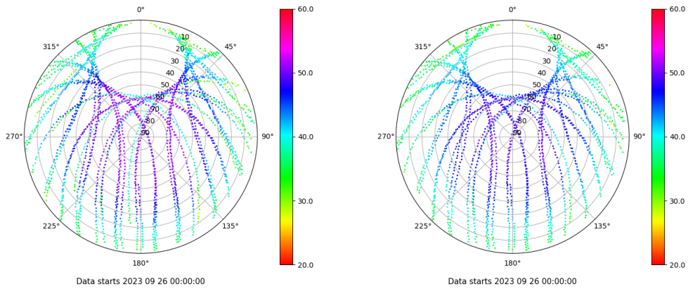
Skyplot for station VIGO. Signal to Noise S1C Data file VIGO00ESP_R_2023269.xtr Skyplot for station VIGO. Signal to Noise S2C Data file VIGO00ESP_R_2023269.xtr
