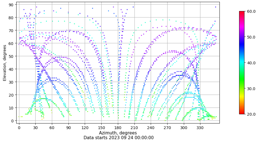
Azimuth-elevation plot for station VIGO. Signal to Noise S1C Data file VIGO00ESP_R_2023267.xtr
