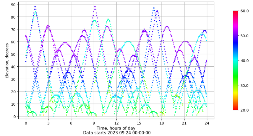
Time-elevation plot for station VIGO. Signal to Noise S1C Data file VIGO00ESP_R_2023267.xtr
