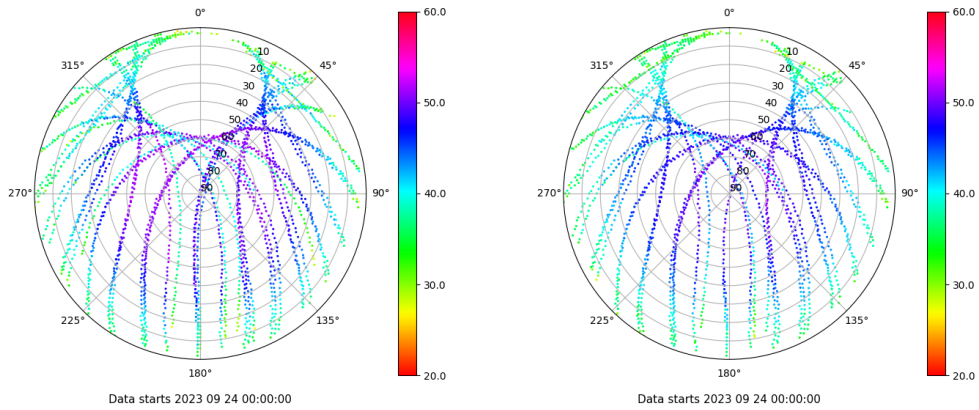
Skyplot for station VIGO. Signal to Noise S1C Data file VIGO00ESP_R_2023267.xtr Skyplot for station VIGO. Signal to Noise S2C Data file VIGO00ESP_R_2023267.xtr
