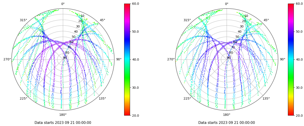
Skyplot for station VIGO. Signal to Noise S1C Data file VIGO00ESP_R_2023264.xtr Skyplot for station VIGO. Signal to Noise S2C Data file VIGO00ESP_R_2023264.xtr
