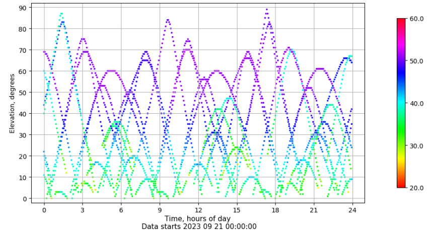
Time-elevation plot for station VIGO. Signal to Noise S1C Data file VIGO00ESP_R_2023264.xtr
