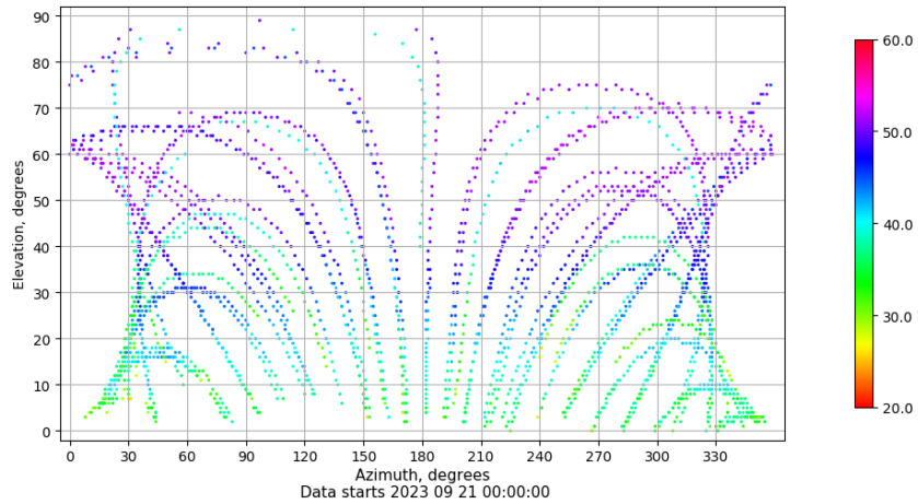
Azimuth-elevation plot for station VIGO. Signal to Noise S1C Data file VIGO00ESP_R_2023264.xtr
