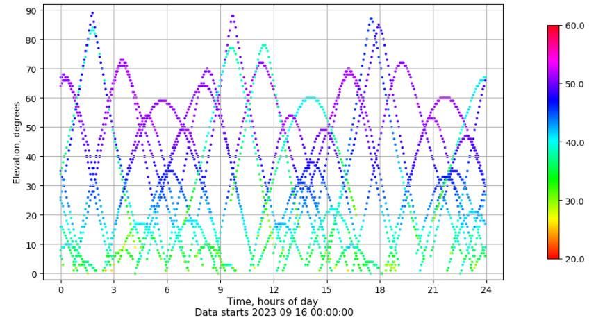
Time-elevation plot for station VIGO. Signal to Noise S1C Data file VIGO00ESP_R_2023259.xtr
