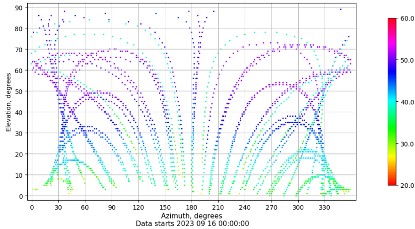
Azimuth-elevation plot for station VIGO. Signal to Noise S1C Data file VIGO00ESP_R_2023259.xtr
