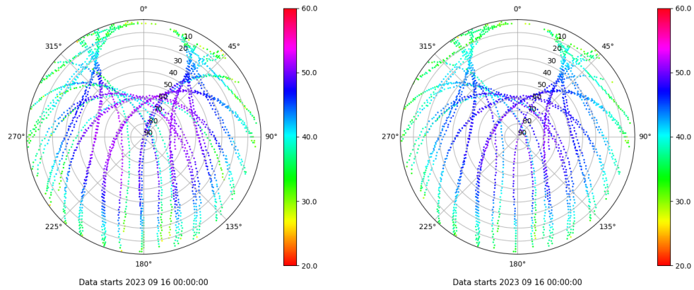
Skyplot for station VIGO. Signal to Noise S1C Data file VIGO00ESP_R_2023259.xtr Skyplot for station VIGO. Signal to Noise S2C Data file VIGO00ESP_R_2023259.xtr
