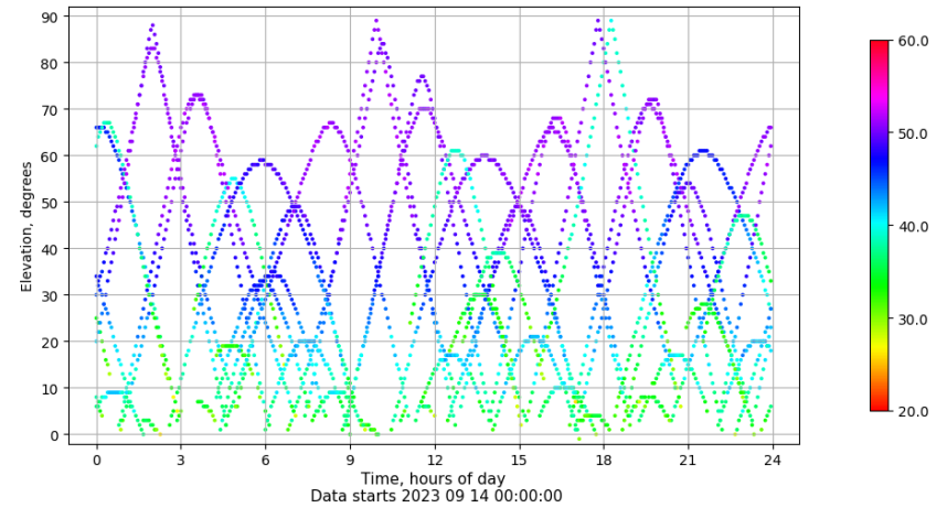
Time-elevation plot for station VIGO. Signal to Noise S1C Data file VIGO00ESP_R_2023257.xtr
