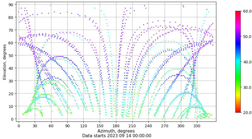
Azimuth-elevation plot for station VIGO. Signal to Noise S1C Data file VIGO00ESP_R_2023257.xtr
