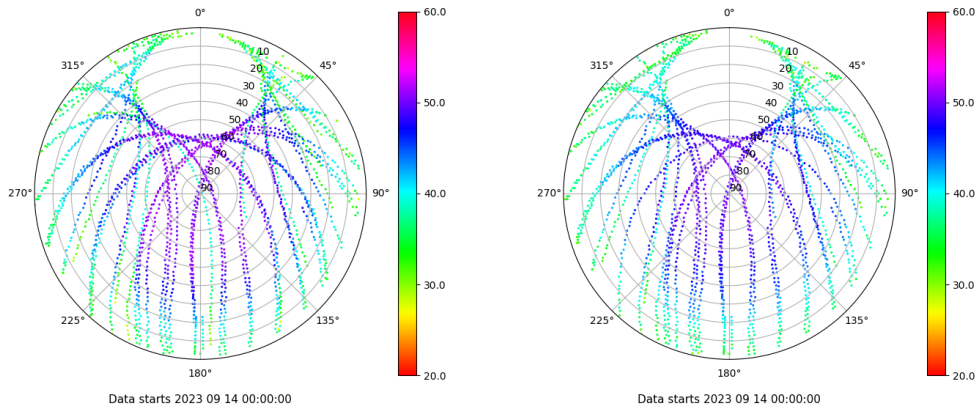
Skyplot for station VIGO. Signal to Noise S1C Data file VIGO00ESP_R_2023257.xtr Skyplot for station VIGO. Signal to Noise S2C Data file VIGO00ESP_R_2023257.xtr
