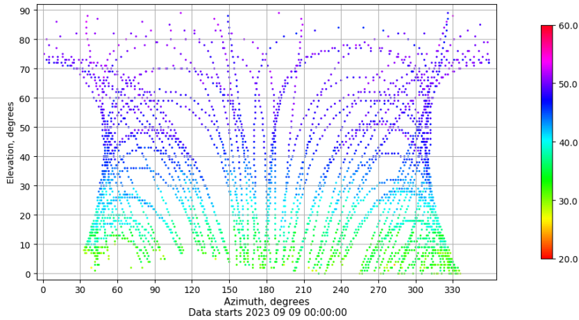
Azimuth-elevation plot for station VIGO. Signal to Noise S1C Data file VIGO00ESP_R_2023252.xtr
