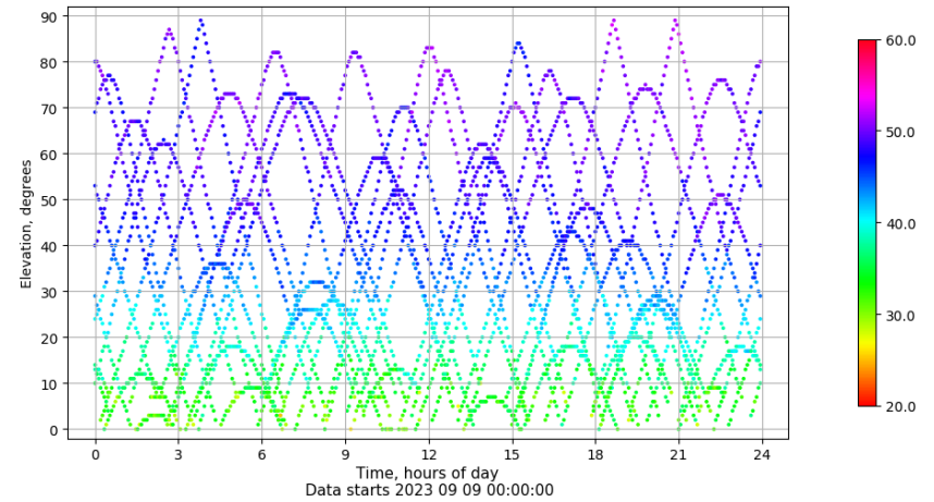
Time-elevation plot for station VIGO. Signal to Noise S1C Data file VIGO00ESP_R_2023252.xtr
