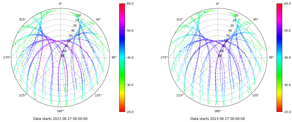
Skyplot for station VIGO. Signal to Noise S1C Data file VIGO00ESP_R_2023239.xtr Skyplot for station VIGO. Signal to Noise S2C Data file VIGO00ESP_R_2023239.xtr
