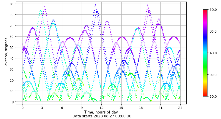
Time-elevation plot for station VIGO. Signal to Noise S1C Data file VIGO00ESP_R_2023239.xtr
