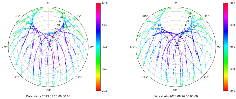
Skyplot for station VIGO. Signal to Noise S1C Data file VIGO00ESP_R_2023238.xtr Skyplot for station VIGO. Signal to Noise S2C Data file VIGO00ESP_R_2023238.xtr
