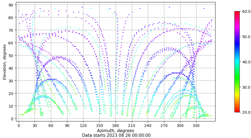
Azimuth-elevation plot for station VIGO. Signal to Noise S1C Data file VIGO00ESP_R_2023238.xtr
