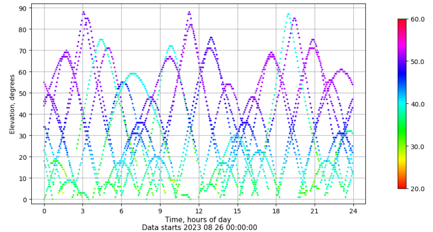
Time-elevation plot for station VIGO. Signal to Noise S1C Data file VIGO00ESP_R_2023238.xtr
