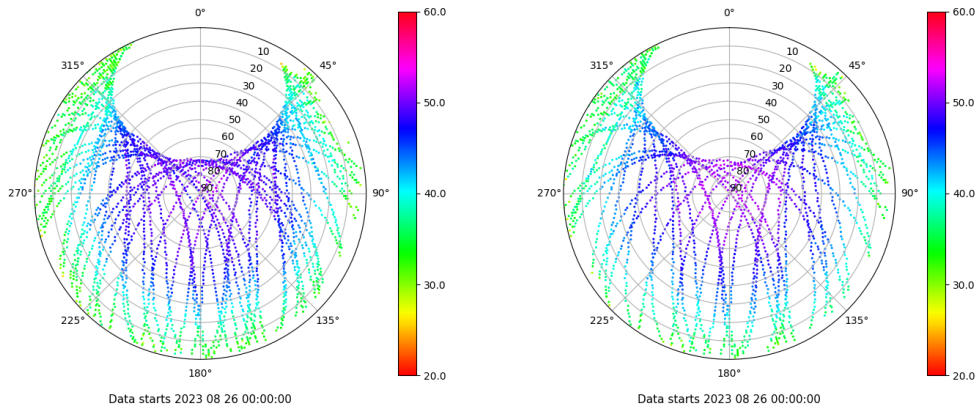
Skyplot for station VIGO. Signal to Noise S1C Data file VIGO00ESP_R_2023238.xtr Skyplot for station VIGO. Signal to Noise S2X Data file VIGO00ESP_R_2023238.xtr
