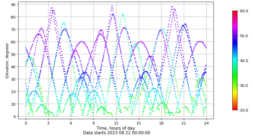
Time-elevation plot for station VIGO. Signal to Noise S1C Data file VIGO00ESP_R_2023234.xtr
