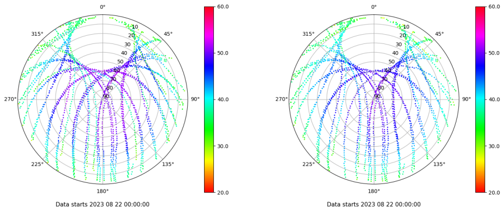
Skyplot for station VIGO. Signal to Noise S1C Data file VIGO00ESP_R_2023234.xtr Skyplot for station VIGO. Signal to Noise S2C Data file VIGO00ESP_R_2023234.xtr
