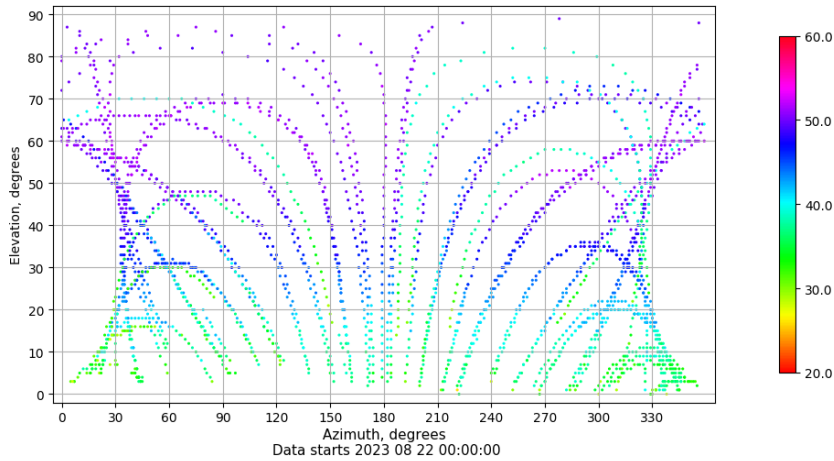
Azimuth-elevation plot for station VIGO. Signal to Noise S1C Data file VIGO00ESP_R_2023234.xtr
