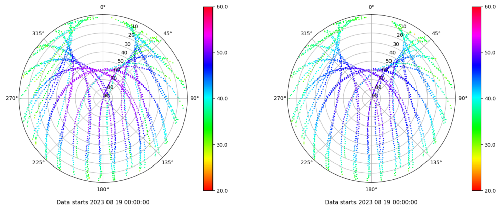
Skyplot for station VIGO. Signal to Noise S1C Data file VIGO00ESP_R_2023231.xtr Skyplot for station VIGO. Signal to Noise S2C Data file VIGO00ESP_R_2023231.xtr
