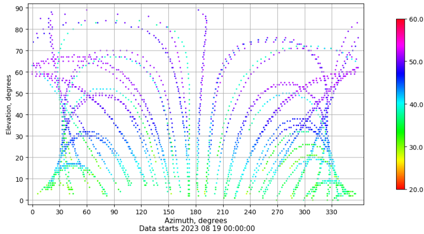
Azimuth-elevation plot for station VIGO. Signal to Noise S1C Data file VIGO00ESP_R_2023231.xtr
