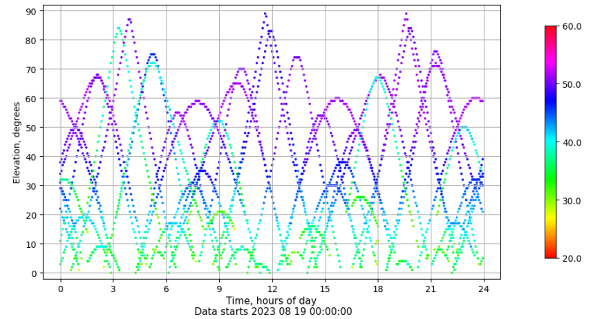
Time-elevation plot for station VIGO. Signal to Noise S1C Data file VIGO00ESP_R_2023231.xtr
