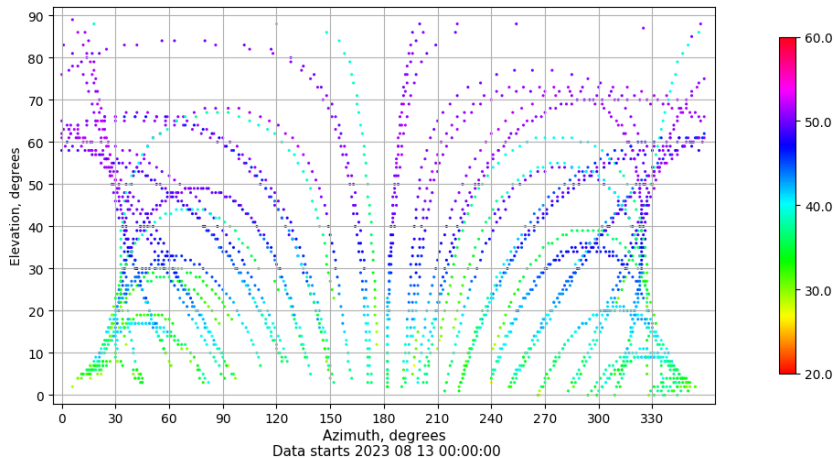
Azimuth-elevation plot for station VIGO. Signal to Noise S1C Data file VIGO00ESP_R_2023225.xtr
