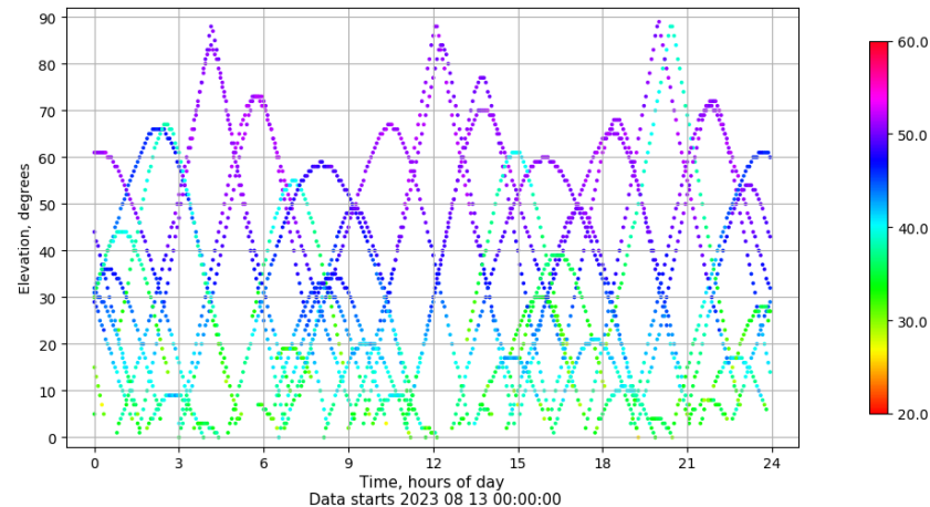
Time-elevation plot for station VIGO. Signal to Noise S1C Data file VIGO00ESP_R_2023225.xtr
