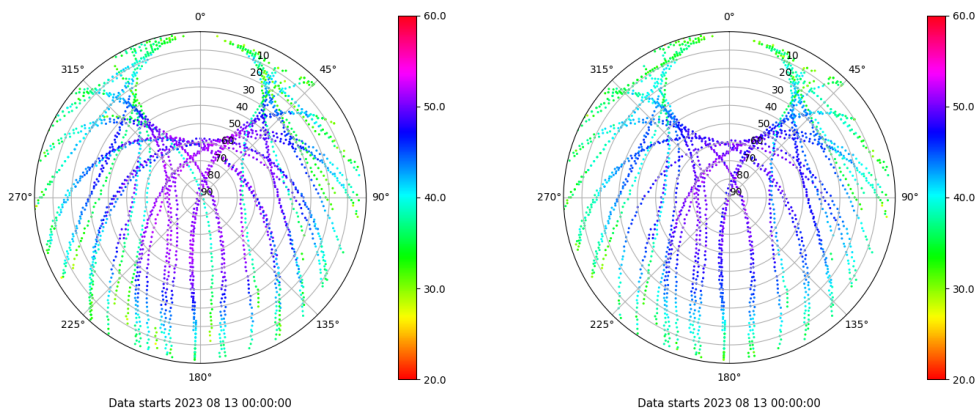
Skyplot for station VIGO. Signal to Noise S1C Data file VIGO00ESP_R_2023225.xtr Skyplot for station VIGO. Signal to Noise S2C Data file VIGO00ESP_R_2023225.xtr
