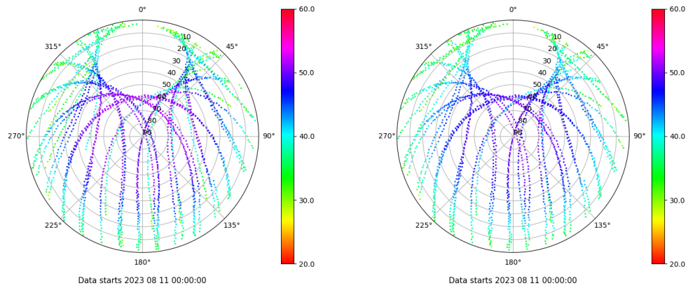
Skyplot for station VIGO. Signal to Noise S1C Data file VIGO00ESP_R_2023223.xtr Skyplot for station VIGO. Signal to Noise S2C Data file VIGO00ESP_R_2023223.xtr
