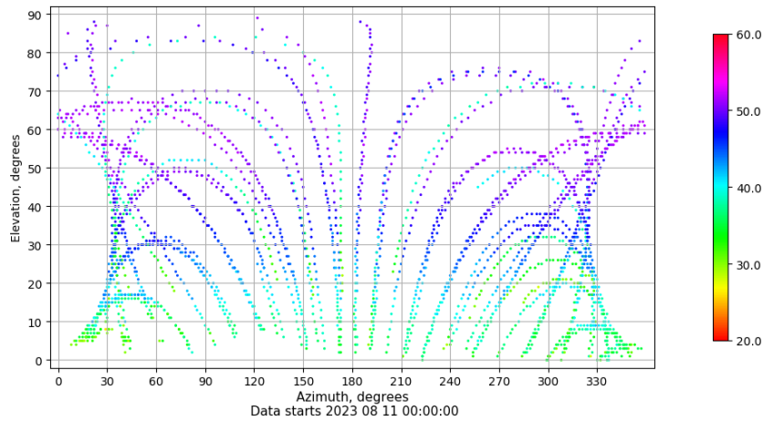
Azimuth-elevation plot for station VIGO. Signal to Noise S1C Data file VIGO00ESP_R_2023223.xtr
