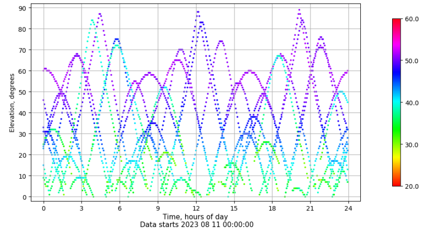
Time-elevation plot for station VIGO. Signal to Noise S1C Data file VIGO00ESP_R_2023223.xtr
