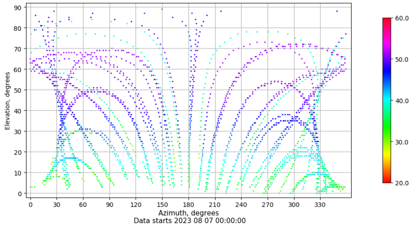
Azimuth-elevation plot for station VIGO. Signal to Noise S1C Data file VIGO00ESP_R_2023219.xtr
