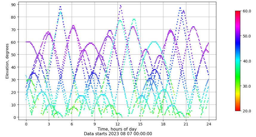
Time-elevation plot for station VIGO. Signal to Noise S1C Data file VIGO00ESP_R_2023219.xtr
