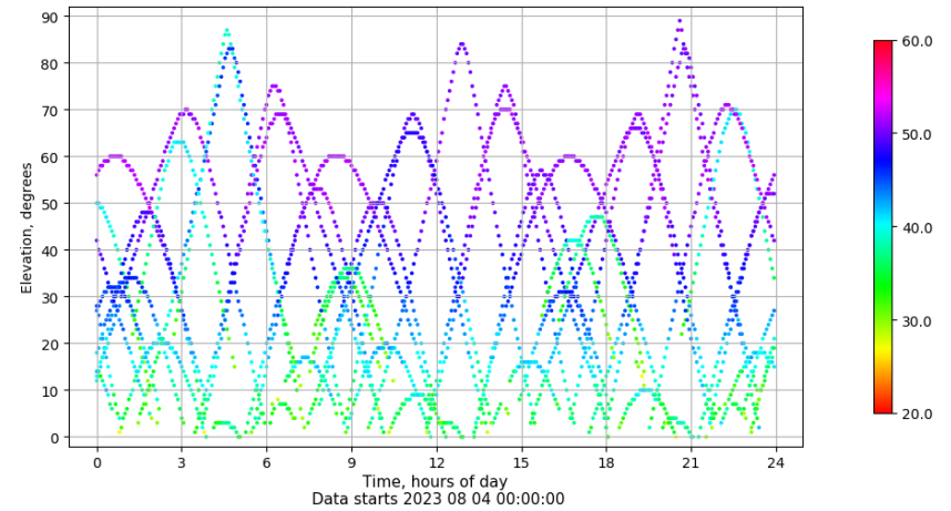
Time-elevation plot for station VIGO. Signal to Noise S1C Data file VIGO00ESP_R_2023216.xtr
