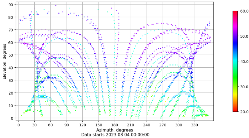
Azimuth-elevation plot for station VIGO. Signal to Noise S1C Data file VIGO00ESP_R_2023216.xtr
