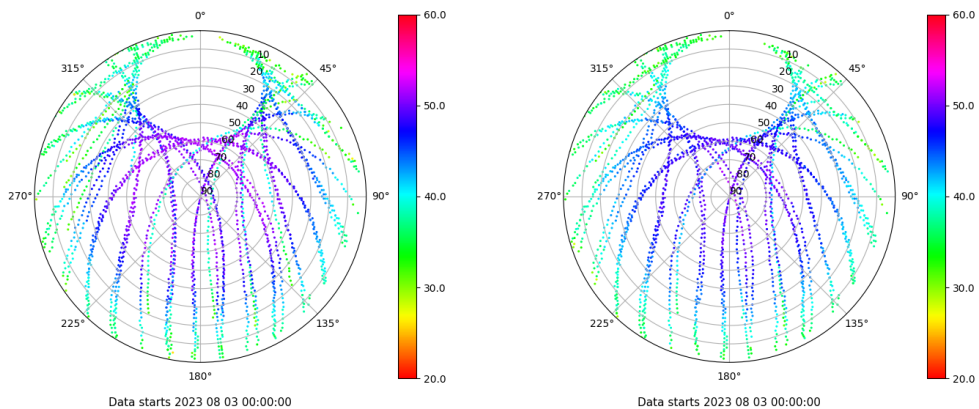
Skyplot for station VIGO. Signal to Noise S1C Data file VIGO00ESP_R_2023215.xtr Skyplot for station VIGO. Signal to Noise S2C Data file VIGO00ESP_R_2023215.xtr
