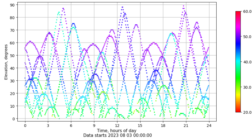
Time-elevation plot for station VIGO. Signal to Noise S1C Data file VIGO00ESP_R_2023215.xtr
