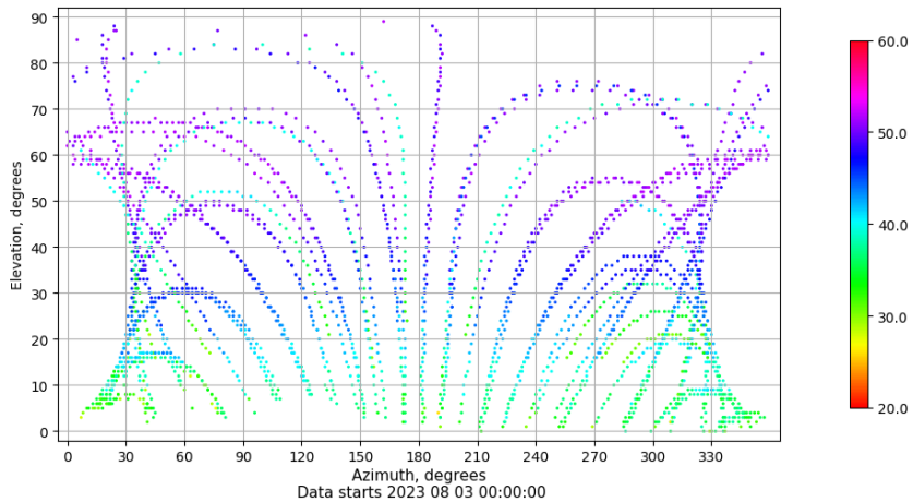
Azimuth-elevation plot for station VIGO. Signal to Noise S1C Data file VIGO00ESP_R_2023215.xtr
