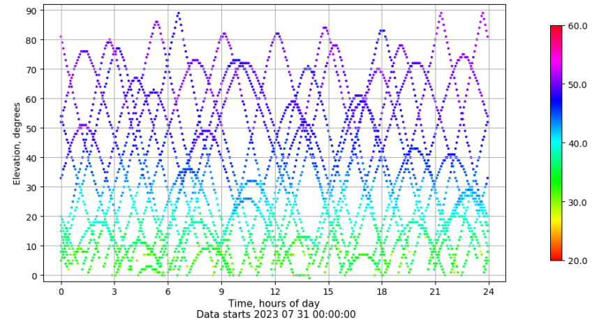
Time-elevation plot for station VIGO. Signal to Noise S1C Data file VIGO00ESP_R_2023212.xtr
