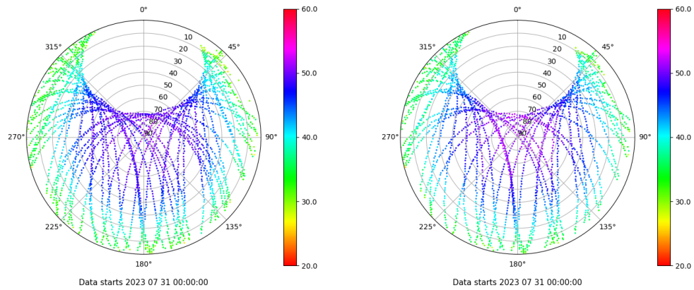
Skyplot for station VIGO. Signal to Noise S1C Data file VIGO00ESP_R_2023212.xtr Skyplot for station VIGO. Signal to Noise S2X Data file VIGO00ESP_R_2023212.xtr
