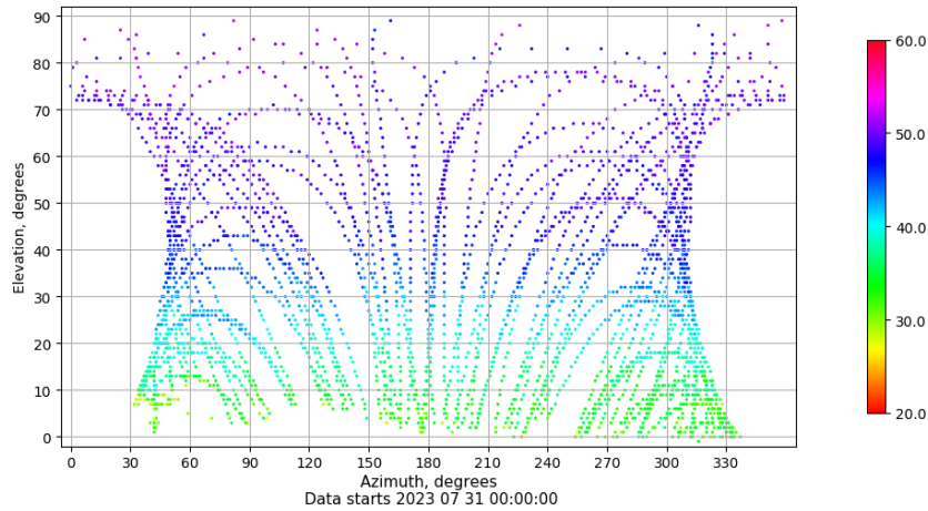
Azimuth-elevation plot for station VIGO. Signal to Noise S1C Data file VIGO00ESP_R_2023212.xtr
