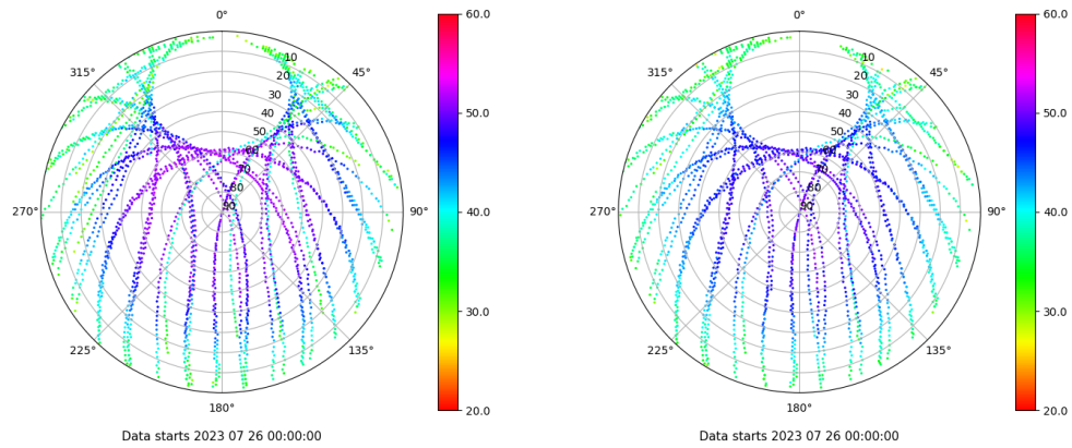
Skyplot for station VIGO. Signal to Noise S1C Data file VIGO00ESP_R_2023207.xtr Skyplot for station VIGO. Signal to Noise S2C Data file VIGO00ESP_R_2023207.xtr
