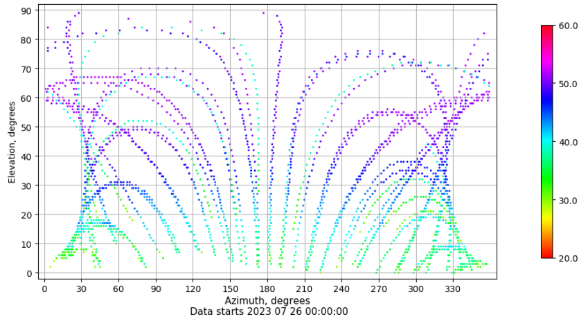
Azimuth-elevation plot for station VIGO. Signal to Noise S1C Data file VIGO00ESP_R_2023207.xtr
