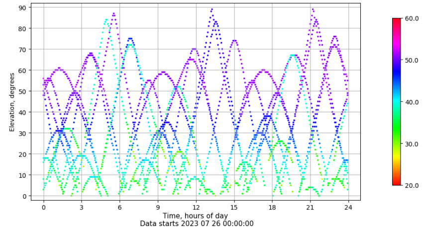
Time-elevation plot for station VIGO. Signal to Noise S1C Data file VIGO00ESP_R_2023207.xtr
