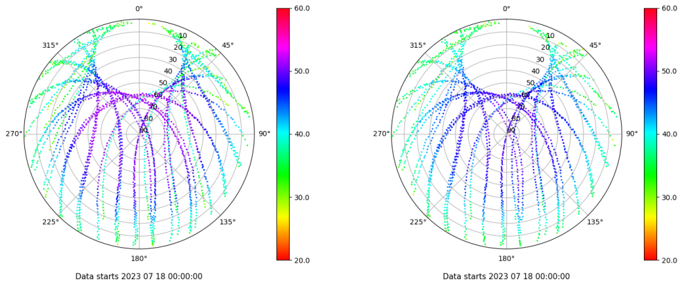
Skyplot for station VIGO. Signal to Noise S1C Data file VIGO00ESP_R_2023199.xtr Skyplot for station VIGO. Signal to Noise S2C Data file VIGO00ESP_R_2023199.xtr
