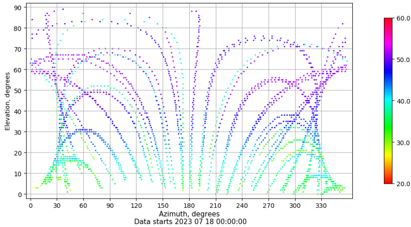
Azimuth-elevation plot for station VIGO. Signal to Noise S1C Data file VIGO00ESP_R_2023199.xtr
