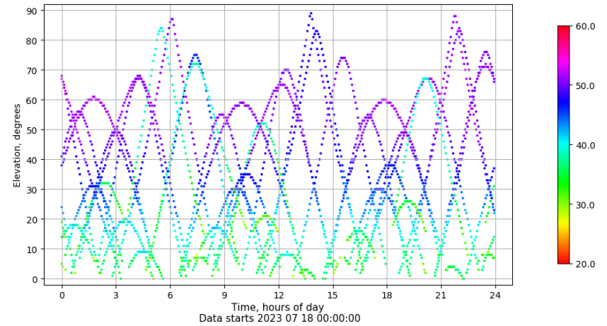
Time-elevation plot for station VIGO. Signal to Noise S1C Data file VIGO00ESP_R_2023199.xtr
