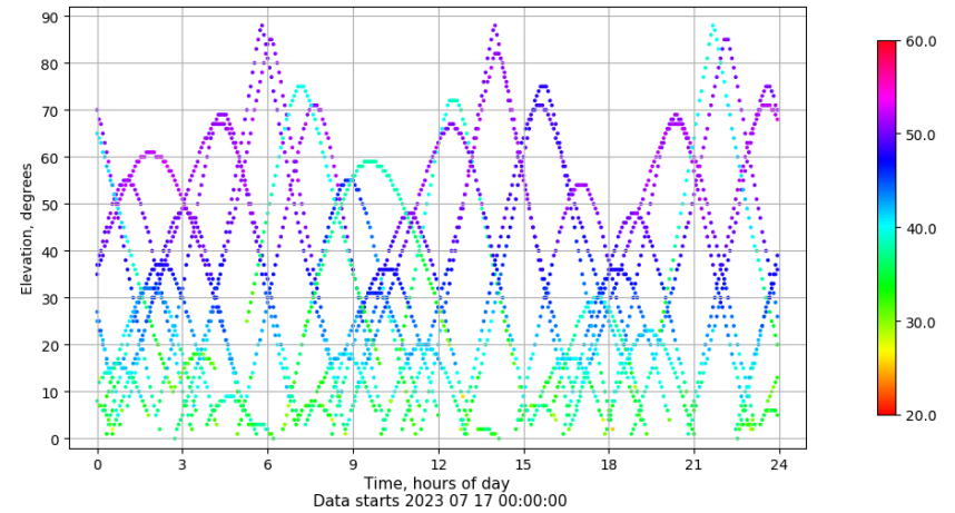
Time-elevation plot for station VIGO. Signal to Noise S1C Data file VIGO00ESP_R_2023198.xtr
