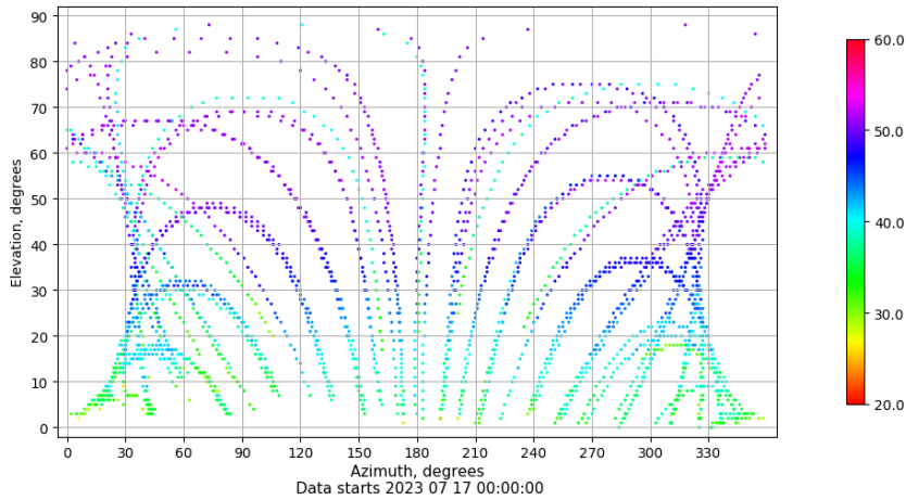
Azimuth-elevation plot for station VIGO. Signal to Noise S1C Data file VIGO00ESP_R_2023198.xtr
