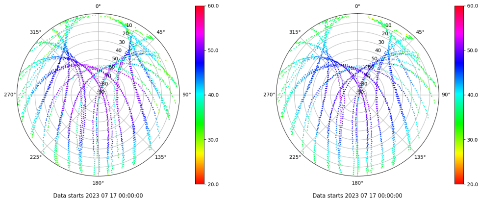
Skyplot for station VIGO. Signal to Noise S1C Data file VIGO00ESP_R_2023198.xtr Skyplot for station VIGO. Signal to Noise S2C Data file VIGO00ESP_R_2023198.xtr
