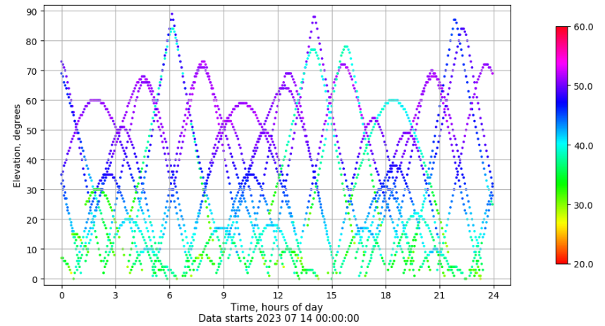
Time-elevation plot for station VIGO. Signal to Noise S1C Data file VIGO00ESP_R_2023195.xtr
