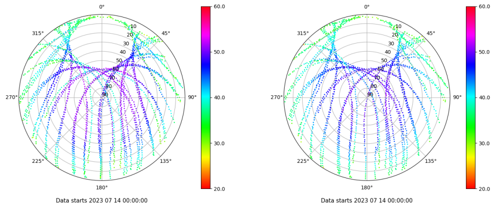
Skyplot for station VIGO. Signal to Noise S1C Data file VIGO00ESP_R_2023195.xtr Skyplot for station VIGO. Signal to Noise S2C Data file VIGO00ESP_R_2023195.xtr
