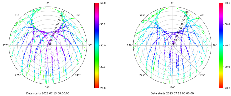
Skyplot for station VIGO. Signal to Noise S1C Data file VIGO00ESP_R_2023194.xtr Skyplot for station VIGO. Signal to Noise S2C Data file VIGO00ESP_R_2023194.xtr
