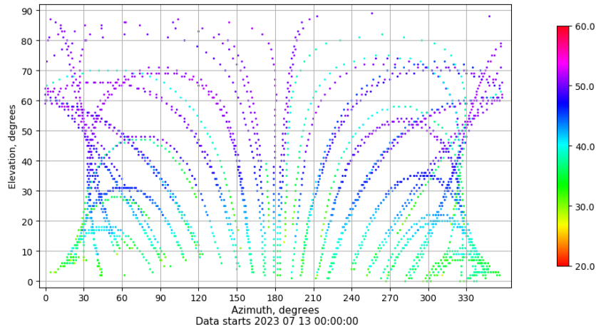
Azimuth-elevation plot for station VIGO. Signal to Noise S1C Data file VIGO00ESP_R_2023194.xtr
