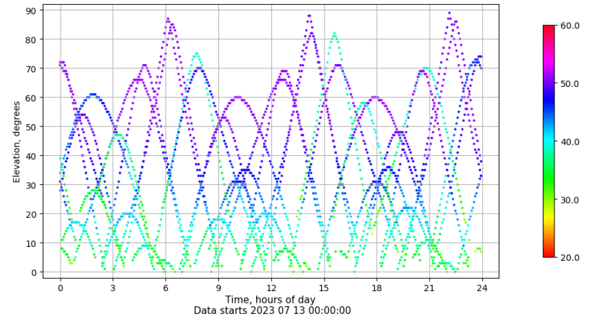
Time-elevation plot for station VIGO. Signal to Noise S1C Data file VIGO00ESP_R_2023194.xtr
