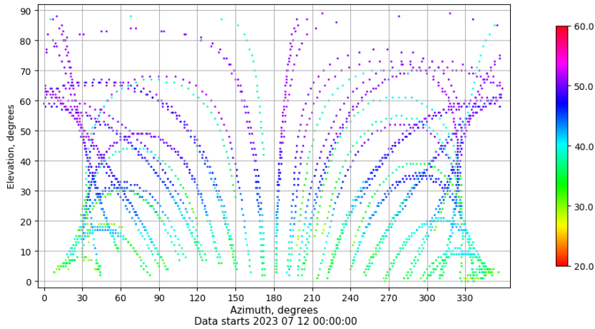
Azimuth-elevation plot for station VIGO. Signal to Noise S1C Data file VIGO00ESP_R_2023193.xtr
