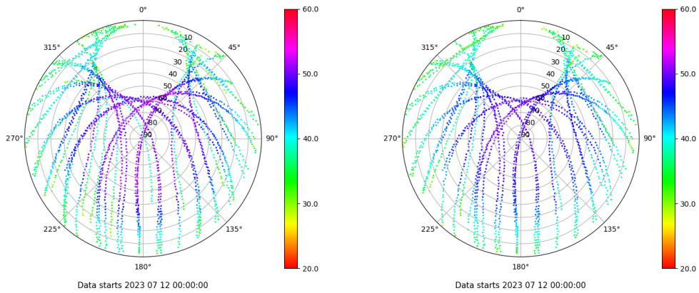
Skyplot for station VIGO. Signal to Noise S1C Data file VIGO00ESP_R_2023193.xtr Skyplot for station VIGO. Signal to Noise S2C Data file VIGO00ESP_R_2023193.xtr
