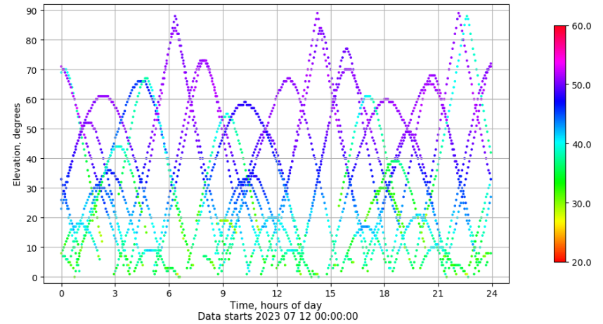
Time-elevation plot for station VIGO. Signal to Noise S1C Data file VIGO00ESP_R_2023193.xtr
