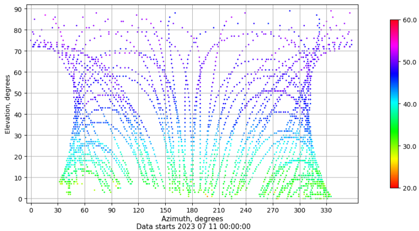
Azimuth-elevation plot for station VIGO. Signal to Noise S1C Data file VIGO00ESP_R_2023192.xtr
