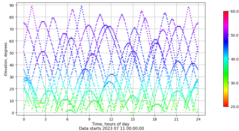
Time-elevation plot for station VIGO. Signal to Noise S1C Data file VIGO00ESP_R_2023192.xtr
