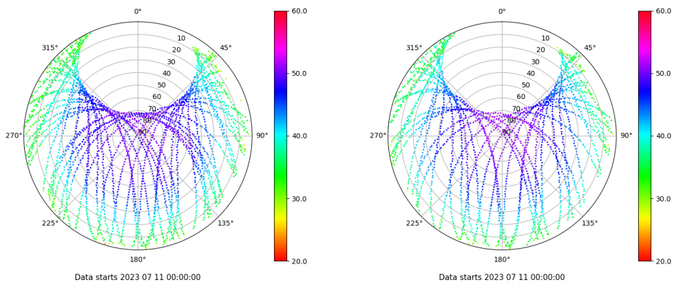
Skyplot for station VIGO. Signal to Noise S1C Data file VIGO00ESP_R_2023192.xtr Skyplot for station VIGO. Signal to Noise S2X Data file VIGO00ESP_R_2023192.xtr
