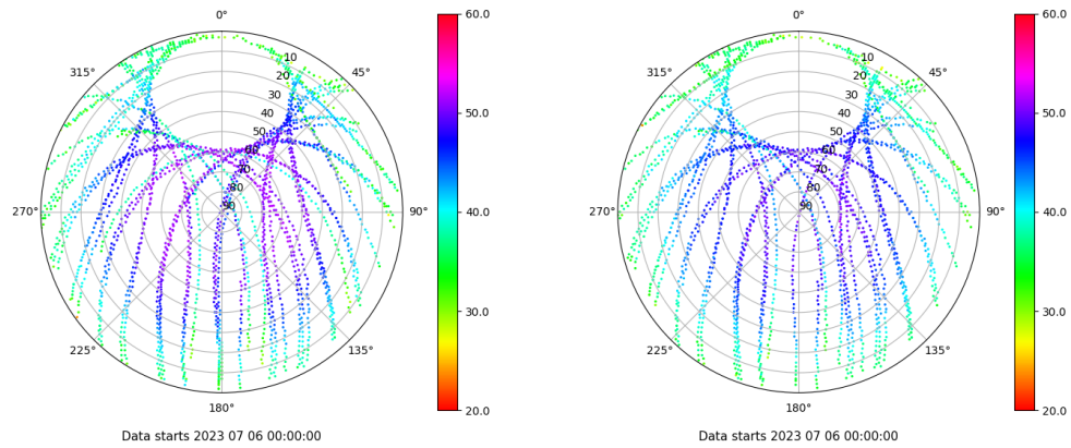
Skyplot for station VIGO. Signal to Noise S1C Data file VIGO00ESP_R_2023187.xtr Skyplot for station VIGO. Signal to Noise S2C Data file VIGO00ESP_R_2023187.xtr
