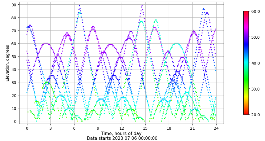
Time-elevation plot for station VIGO. Signal to Noise S1C Data file VIGO00ESP_R_2023187.xtr
