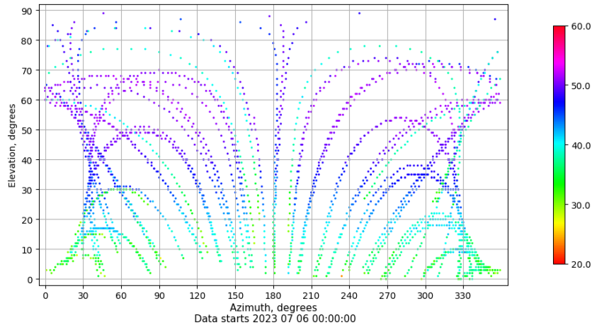
Azimuth-elevation plot for station VIGO. Signal to Noise S1C Data file VIGO00ESP_R_2023187.xtr
