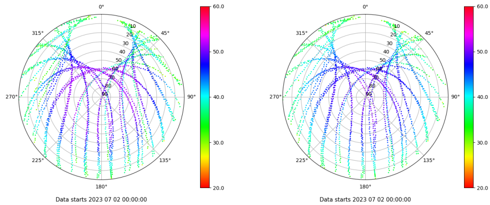
Skyplot for station VIGO. Signal to Noise S1C Data file VIGO00ESP_R_2023183.xtr Skyplot for station VIGO. Signal to Noise S2C Data file VIGO00ESP_R_2023183.xtr
