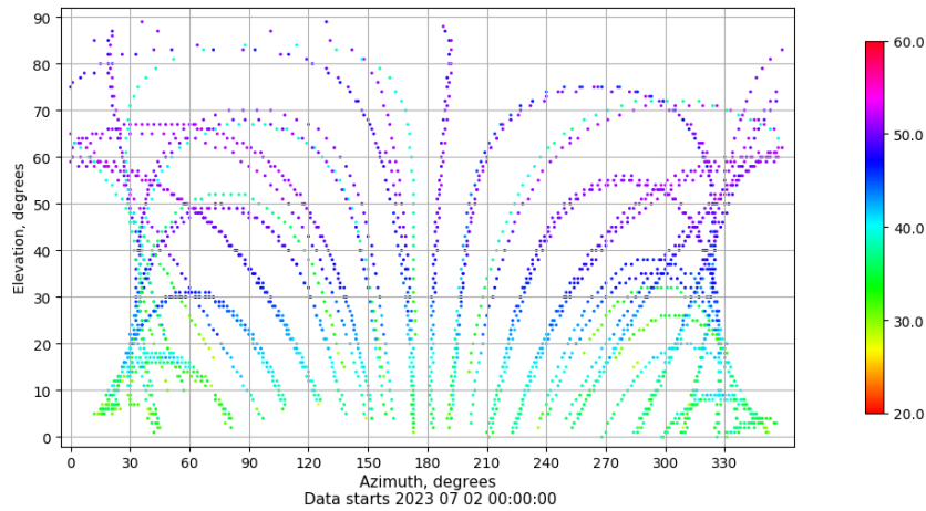
Azimuth-elevation plot for station VIGO. Signal to Noise S1C Data file VIGO00ESP_R_2023183.xtr
