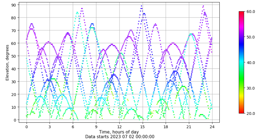
Time-elevation plot for station VIGO. Signal to Noise S1C Data file VIGO00ESP_R_2023183.xtr
