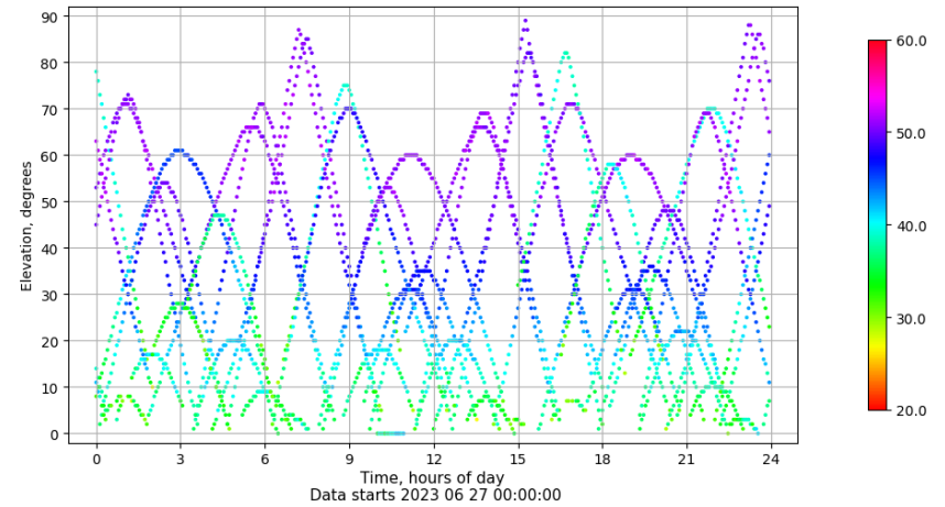
Time-elevation plot for station VIGO. Signal to Noise S1C Data file VIGO00ESP_R_2023178.xtr
