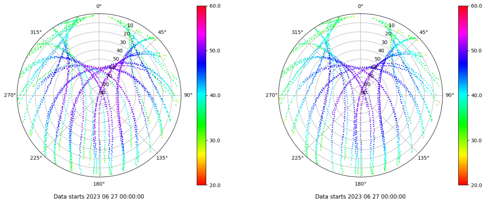
Skyplot for station VIGO. Signal to Noise S1C Data file VIGO00ESP_R_2023178.xtr Skyplot for station VIGO. Signal to Noise S2C Data file VIGO00ESP_R_2023178.xtr
