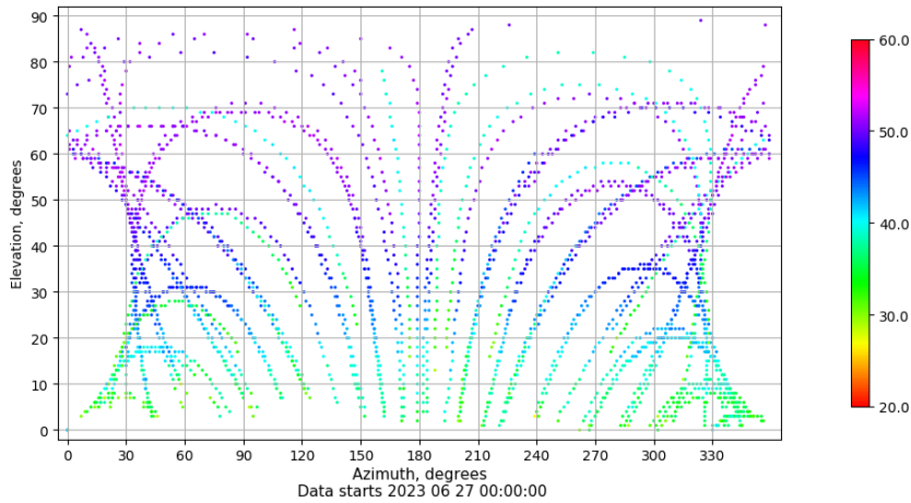
Azimuth-elevation plot for station VIGO. Signal to Noise S1C Data file VIGO00ESP_R_2023178.xtr
