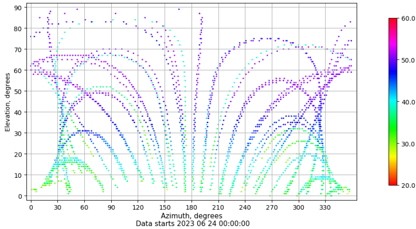
Azimuth-elevation plot for station VIGO. Signal to Noise S1C Data file VIGO00ESP_R_2023175.xtr
