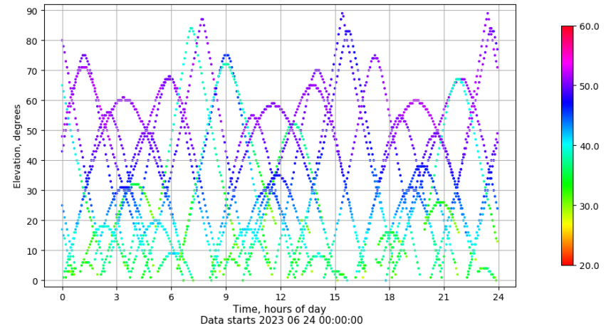
Time-elevation plot for station VIGO. Signal to Noise S1C Data file VIGO00ESP_R_2023175.xtr
