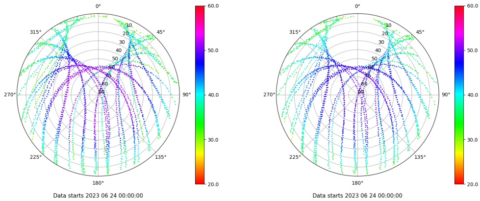
Skyplot for station VIGO. Signal to Noise S1C Data file VIGO00ESP_R_2023175.xtr Skyplot for station VIGO. Signal to Noise S2C Data file VIGO00ESP_R_2023175.xtr
