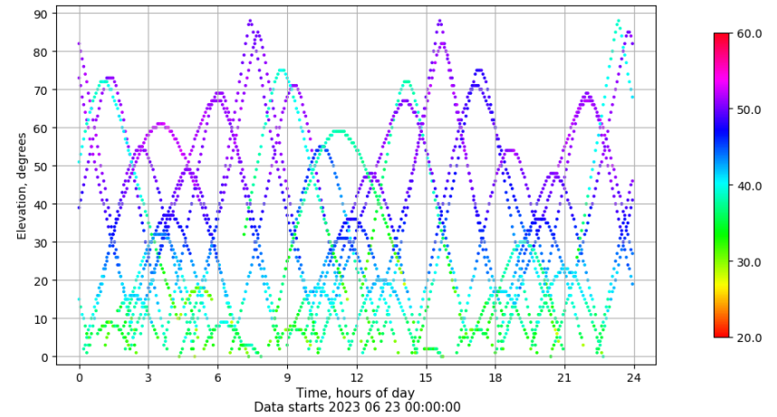
Time-elevation plot for station VIGO. Signal to Noise S1C Data file VIGO00ESP_R_2023174.xtr
