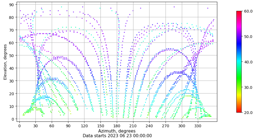
Azimuth-elevation plot for station VIGO. Signal to Noise S1C Data file VIGO00ESP_R_2023174.xtr
