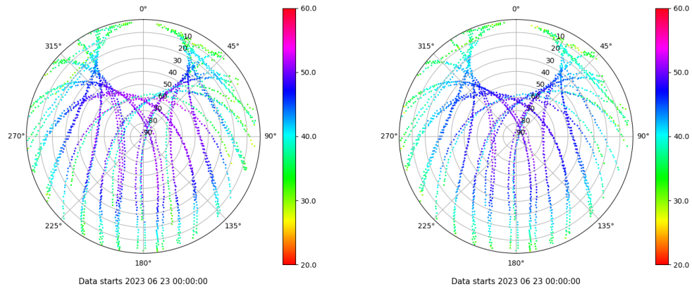
Skyplot for station VIGO. Signal to Noise S1C Data file VIGO00ESP_R_2023174.xtr Skyplot for station VIGO. Signal to Noise S2C Data file VIGO00ESP_R_2023174.xtr
