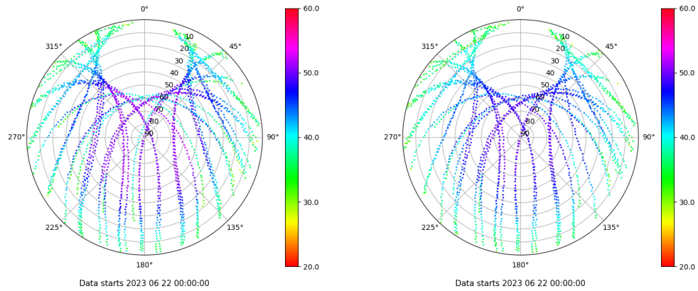
Skyplot for station VIGO. Signal to Noise S1C Data file VIGO00ESP_R_2023173.xtr Skyplot for station VIGO. Signal to Noise S2C Data file VIGO00ESP_R_2023173.xtr
