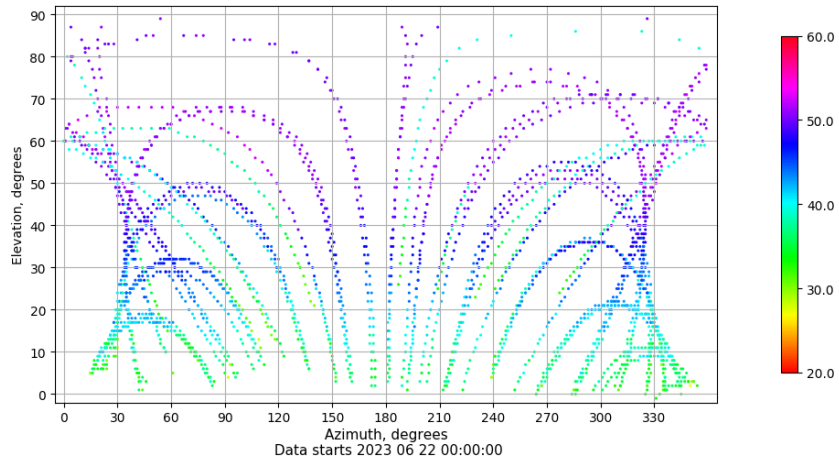
Azimuth-elevation plot for station VIGO. Signal to Noise S1C Data file VIGO00ESP_R_2023173.xtr
