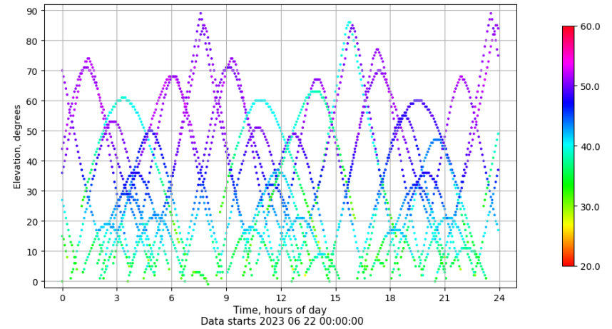
Time-elevation plot for station VIGO. Signal to Noise S1C Data file VIGO00ESP_R_2023173.xtr
