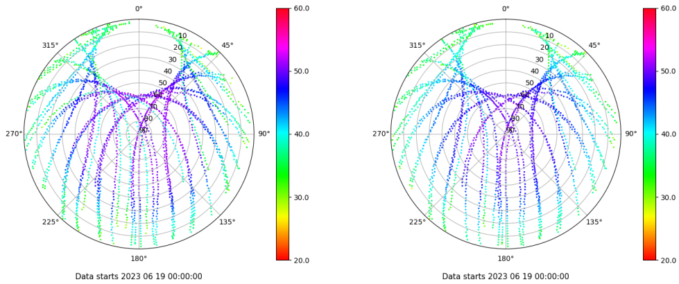
Skyplot for station VIGO. Signal to Noise S1C Data file VIGO00ESP_R_2023170.xtr Skyplot for station VIGO. Signal to Noise S2C Data file VIGO00ESP_R_2023170.xtr
