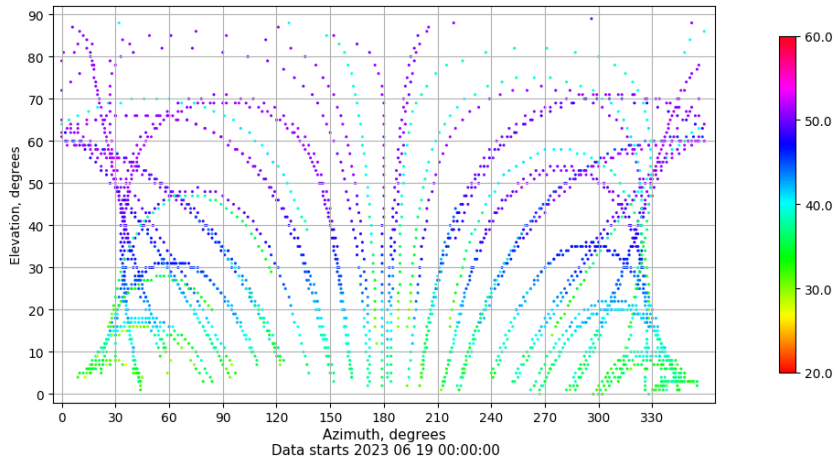
Azimuth-elevation plot for station VIGO. Signal to Noise S1C Data file VIGO00ESP_R_2023170.xtr
