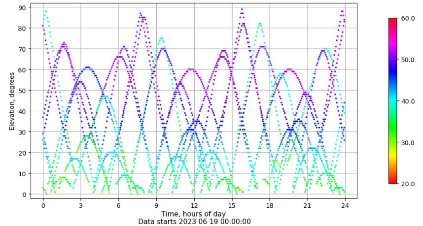
Time-elevation plot for station VIGO. Signal to Noise S1C Data file VIGO00ESP_R_2023170.xtr
