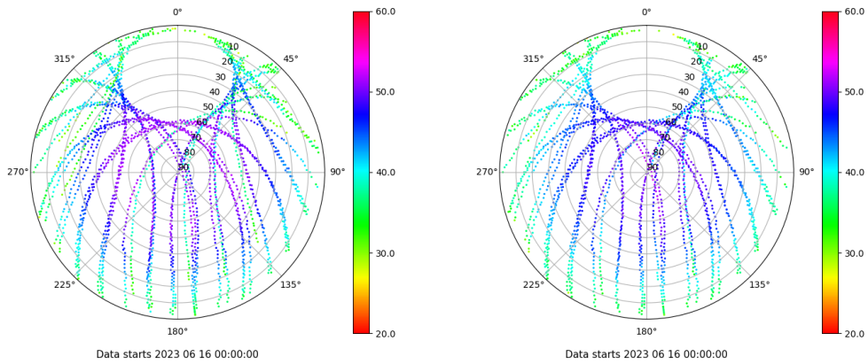
Skyplot for station VIGO. Signal to Noise S1C Data file VIGO00ESP_R_2023167.xtr Skyplot for station VIGO. Signal to Noise S2C Data file VIGO00ESP_R_2023167.xtr
