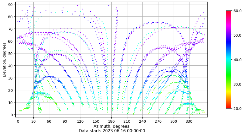
Azimuth-elevation plot for station VIGO. Signal to Noise S1C Data file VIGO00ESP_R_2023167.xtr
