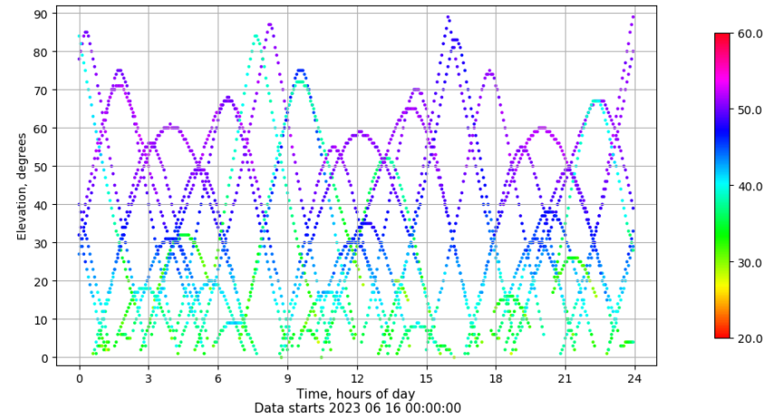
Time-elevation plot for station VIGO. Signal to Noise S1C Data file VIGO00ESP_R_2023167.xtr
