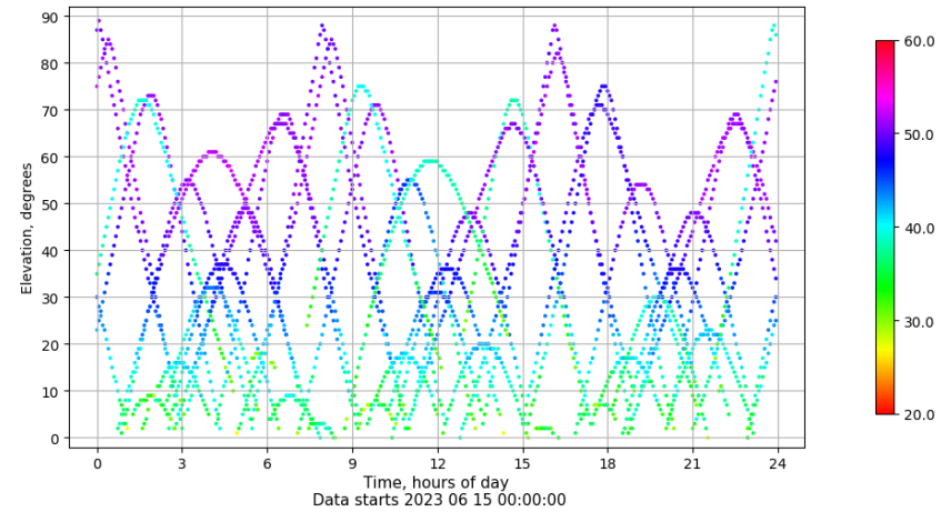
Time-elevation plot for station VIGO. Signal to Noise S1C Data file VIGO00ESP_R_2023166.xtr
