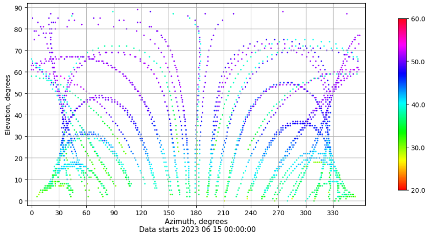
Azimuth-elevation plot for station VIGO. Signal to Noise S1C Data file VIGO00ESP_R_2023166.xtr
