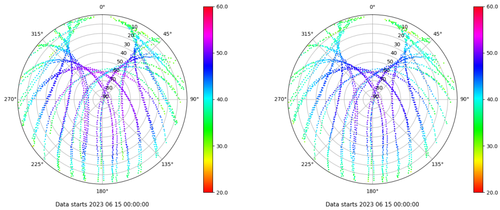
Skyplot for station VIGO. Signal to Noise S1C Data file VIGO00ESP_R_2023166.xtr Skyplot for station VIGO. Signal to Noise S2C Data file VIGO00ESP_R_2023166.xtr
