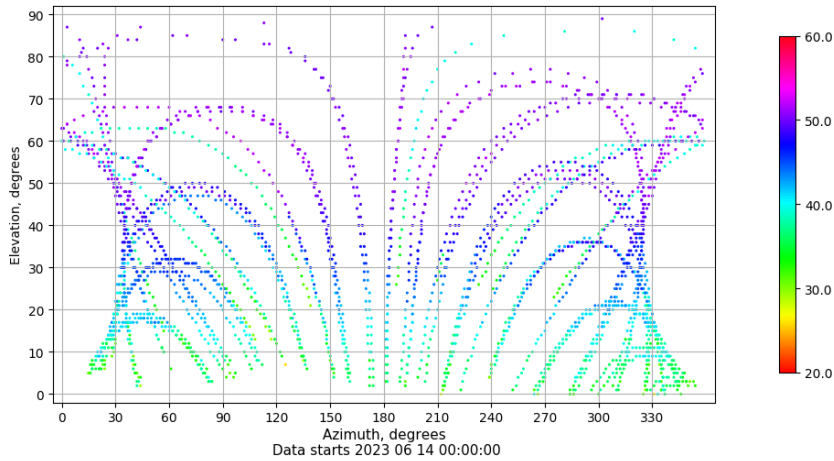
Azimuth-elevation plot for station VIGO. Signal to Noise S1C Data file VIGO00ESP_R_2023165.xtr
