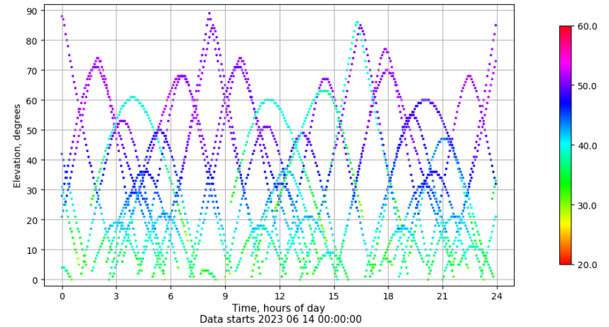
Time-elevation plot for station VIGO. Signal to Noise S1C Data file VIGO00ESP_R_2023165.xtr
