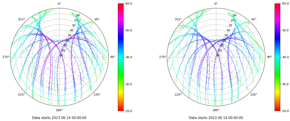
Skyplot for station VIGO. Signal to Noise S1C Data file VIGO00ESP_R_2023165.xtr Skyplot for station VIGO. Signal to Noise S2C Data file VIGO00ESP_R_2023165.xtr
