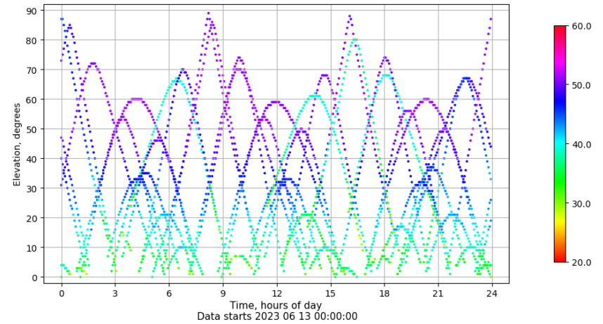
Time-elevation plot for station VIGO. Signal to Noise S1C Data file VIGO00ESP_R_2023164.xtr
