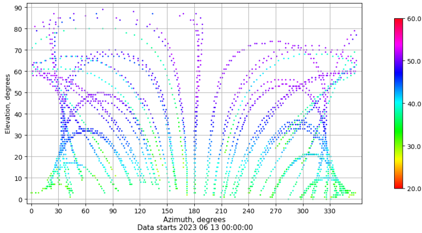
Azimuth-elevation plot for station VIGO. Signal to Noise S1C Data file VIGO00ESP_R_2023164.xtr
